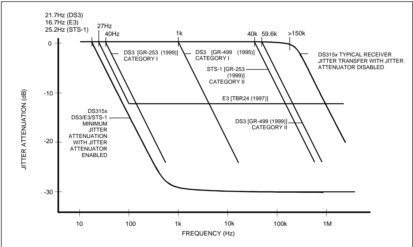
Figure 9-1. Jitter Attenuation/Jitter Transfer
