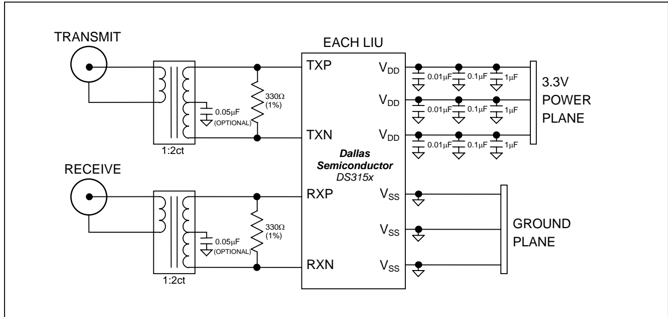
Figure 1-1. External Connections
