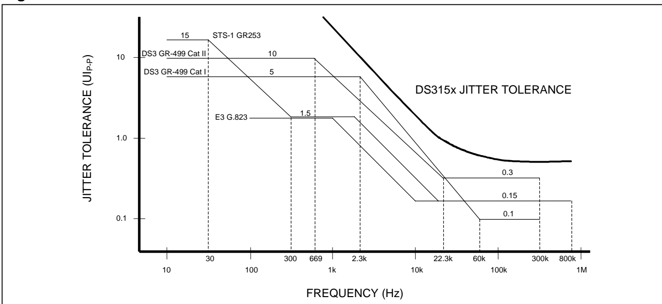
Figure 6-1. Receiver Jitter Tolerance
