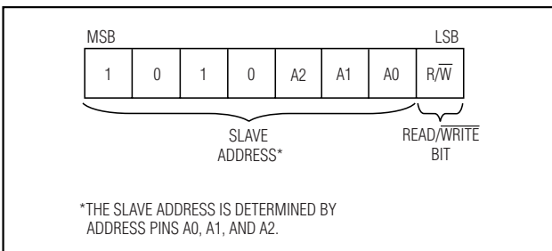
Figure 1. DS3906 Slave Address Byte
