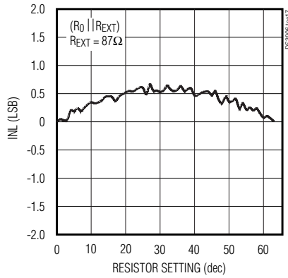
INL vs. RESISTOR SETTING FOR (R 0 || R EXT )
