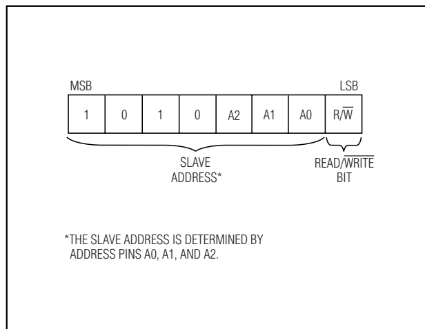
Figure 1. DS3908 Slave Address Byte
