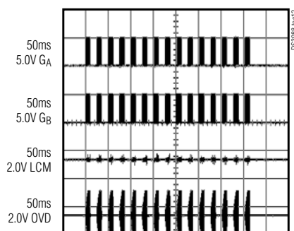
LAMP STRIKE WITH OPEN LAMP AUTORETRY ENABLED
