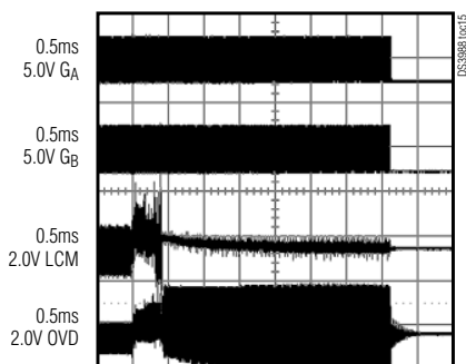
LAMP-OUT (LAMP OPENED) AUTORETRY DISABLED
