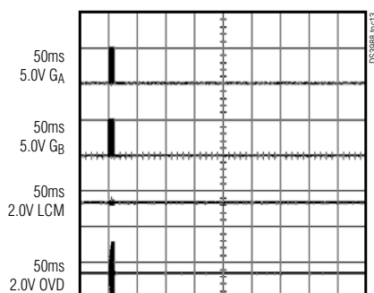
LAMP STRIKE WITH OPEN LAMP AUTORETRY DISABLED
