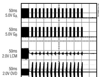
LAMP-OUT (LAMP OPENED) AUTORETRY ENABLED
