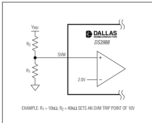
Figure 7. Setting the SVM Threshold Voltage
