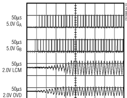
SOFT-START AT V_{INV} = 18V
