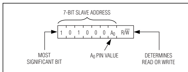
Figure 10. DS3988's Slave Address Byte
