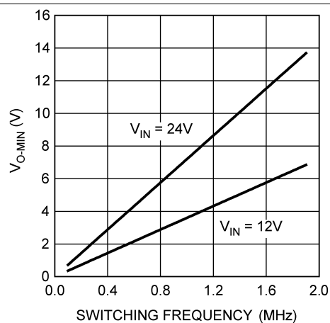
Figure 14. V_{O-MIN} vs f_{SW} , LM3402 ( T_A = 25^\circ\text{C} )
