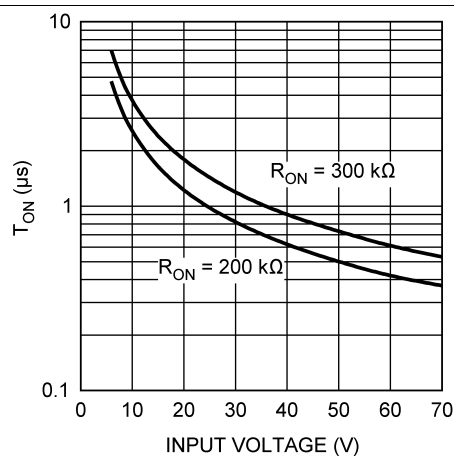
Figure 8. T_{ON} vs V_{IN} ( T_A = 25^\circ\text{C} )
