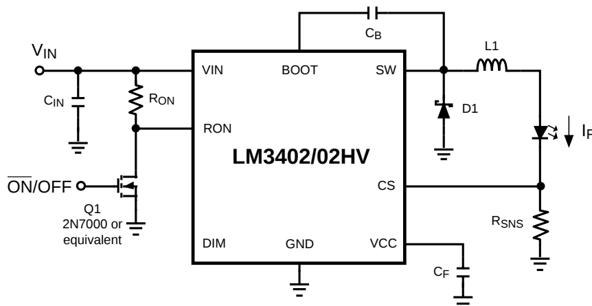
Figure 19. Low Power Shutdown
