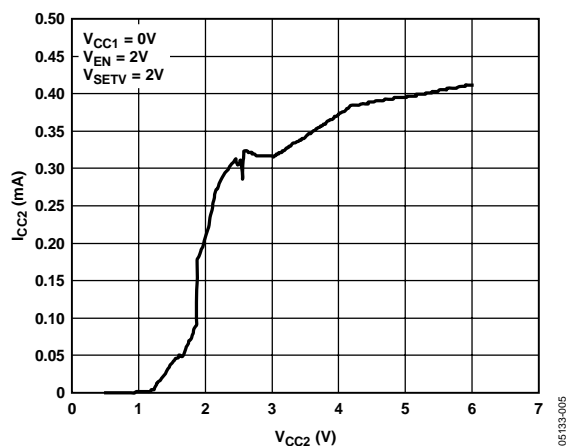
Figure 9. I_{CC2} vs. V_{CC2}
