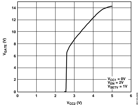
Figure 13. V_{GATE} vs. V_{CC2}
