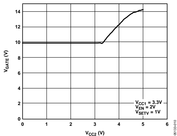
Figure 14. V_{GATE} vs. V_{CC2}
