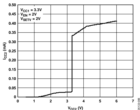
Figure 10. I_{CC2} vs. V_{CC2}
