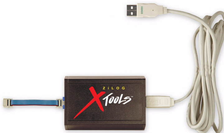
Figure 1. Opto-Isolated USB Smart Cable
