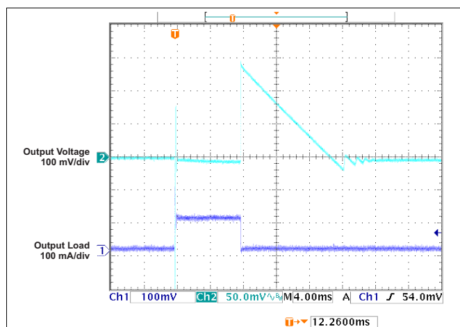
Figure 19. Load Transient Response vs Time ( V_{OUT} = 5V , C_L = 10\mu F )
