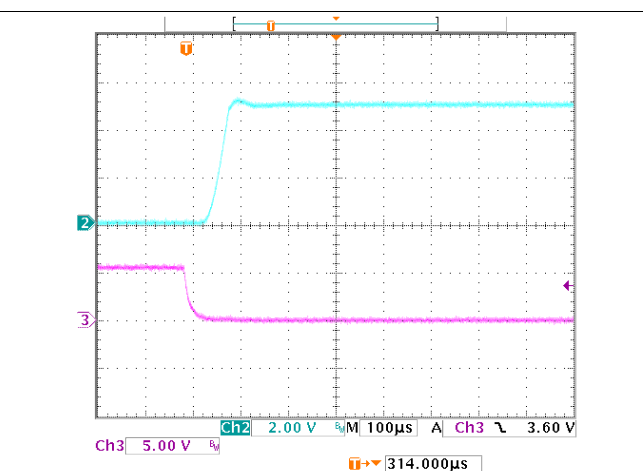
Figure 20. Enable Transient Response vs Time ( I_L = 1mA , C_L = 1\mu F )
