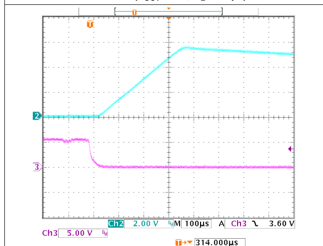
Figure 21. Enable Transient Response vs Time ( I_L = 1mA , C_L = 10\mu F )
