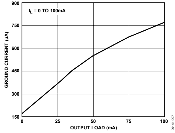
Figure 7. Quiescent Current vs. Load Current
