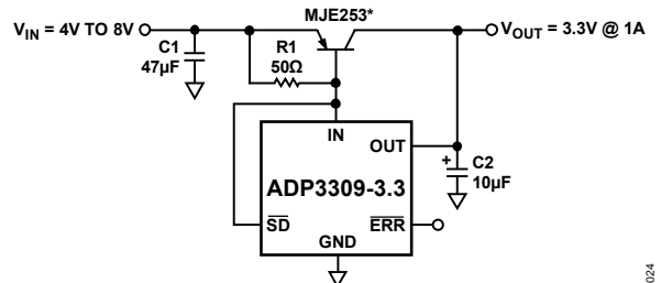
Figure 24. Higher Output Current Linear Regulator
