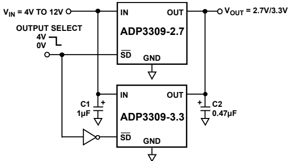
Figure 23. Crossover Switch
