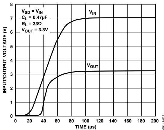
Figure 12. Power-Up Overshoot
