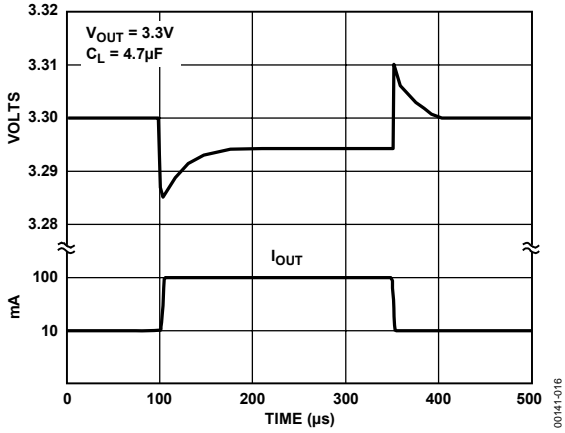
Figure 16. Load Transient
