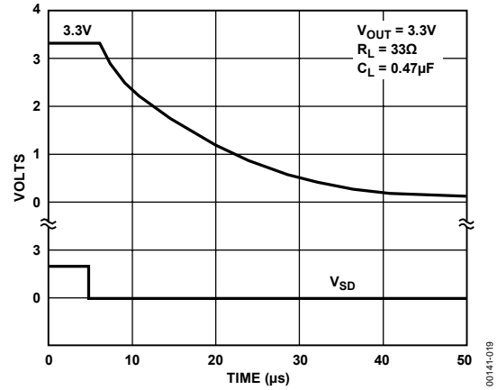
Figure 19. Turn-Off
