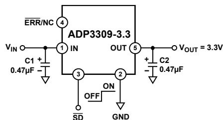
Figure 2. Typical Application Circuit
