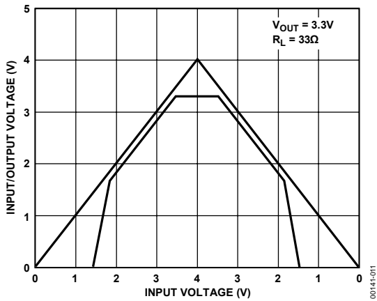
Figure 11. Power-Up/Power-Down
