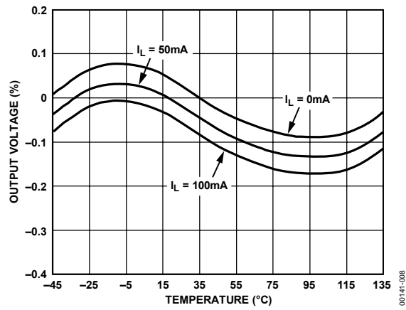
Figure 8. Output Voltage Variation % vs. Temperature
