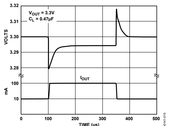
Figure 15. Load Transient
