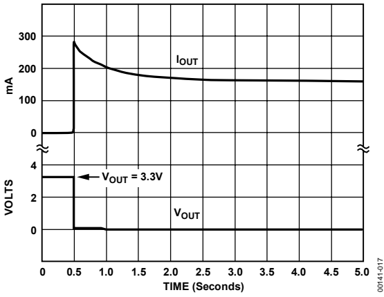
Figure 17. Short-Circuit Current
