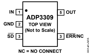
Figure 3. Pin Configuration
