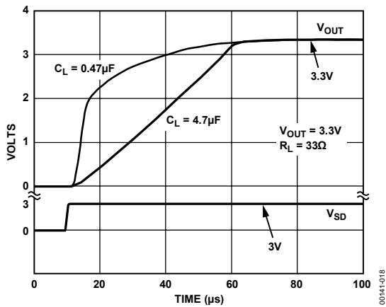
Figure 18. Turn-On
