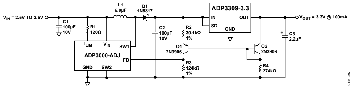
Figure 25. Constant Dropout Post Regulator
