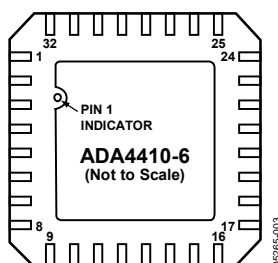
Figure 3. 32-Lead LFCSP Pin Configuration, Top View
