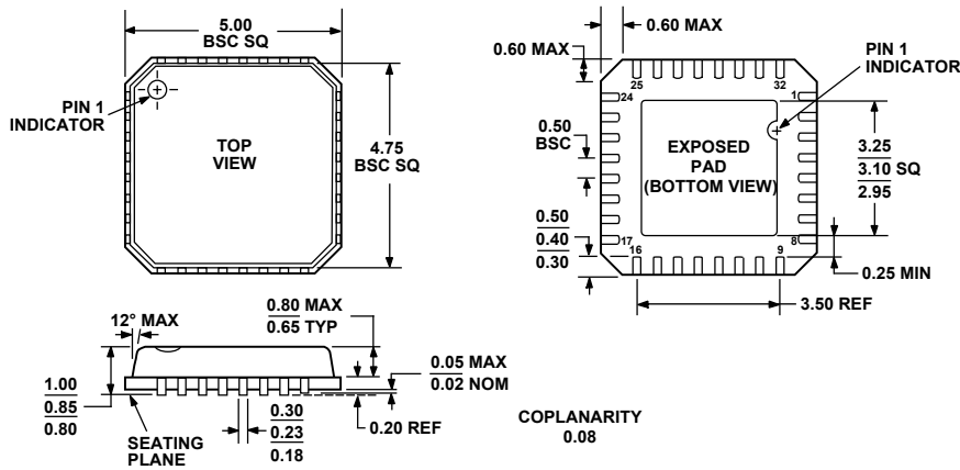
COMPLIANT TO JEDEC STANDARDS MO-220-VHHD-2 Figure 28. 32-Lead Lead Frame Chip Scale Package [LFCSP_VQ] 5 mm × 5 mm Body, Very Thin Quad (CP-32-2) Dimensions shown in millimeters
