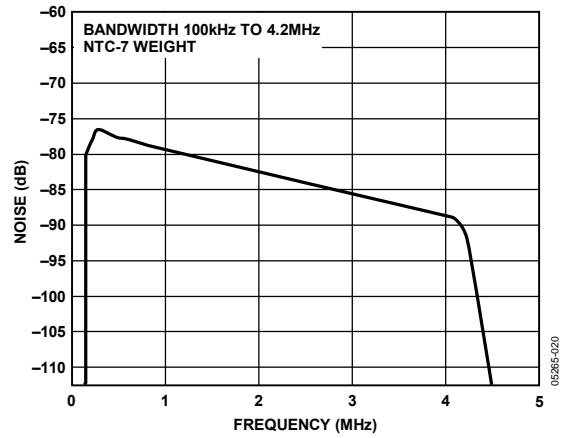
Figure 13. CV Noise Spectrum
