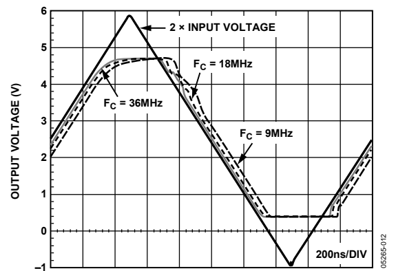
Figure 21. Overdrive Recovery vs. Cutoff Frequency
