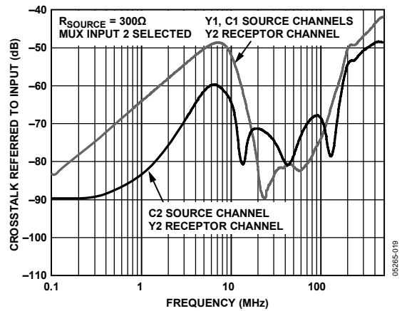
Figure 14. SD Channel Crosstalk vs. Frequency
