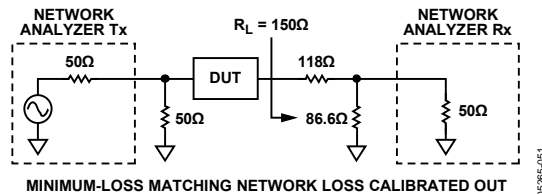
Figure 22. Basic Test Circuit for Swept Frequency Measurements
