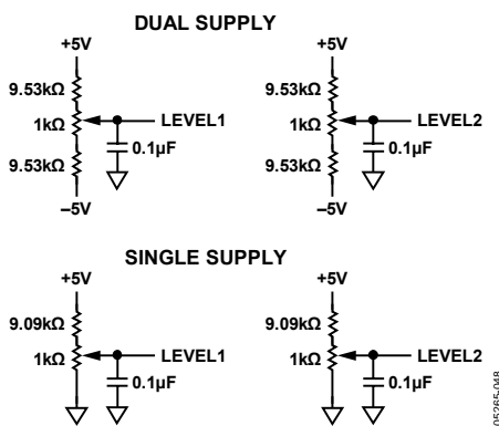
Figure 23. Generating Fully Adjustable Output Offsets
