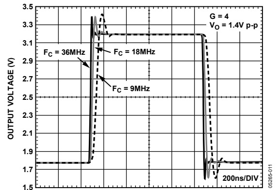
Figure 20. Transient Response vs. Cutoff Frequency ( G = \times 4 )
