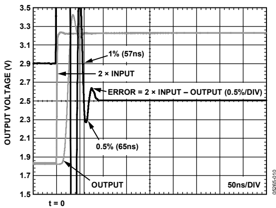
Figure 18. Settling Time
