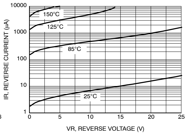
Figure 2. Leakage Current
