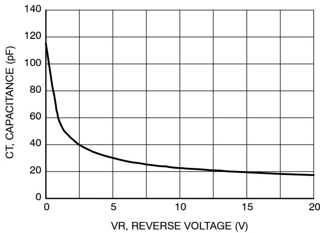
Figure 3. Total Capacitance
