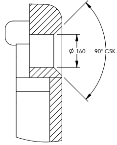
DETAIL D SCALE 6 : 1
