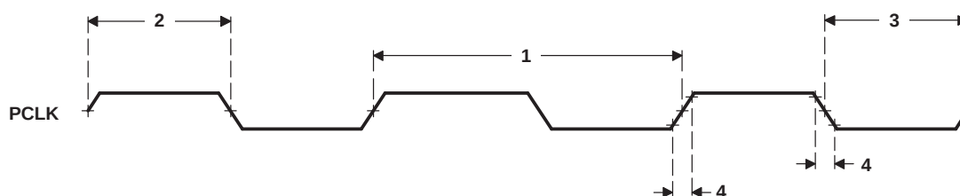
Figure 6-46. VPFE PCLK Timing
