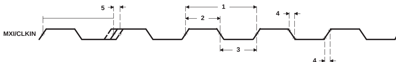
Figure 6-15. M24XI Timing
