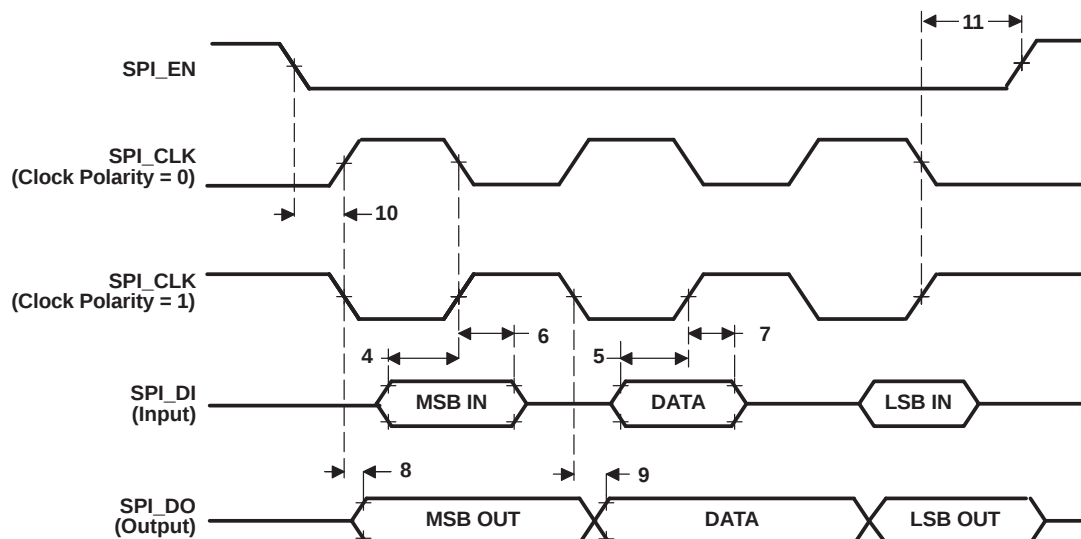
Figure 6-63. SPI Master Mode External Timing (Clock Phase = 0)
