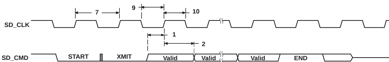
Figure 6-43. MMC/SD/SDIO Card Response Timing
