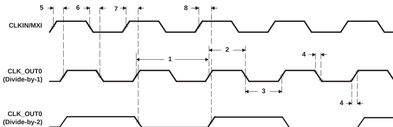
Figure 6-16. CLK_OUT0 Timing
