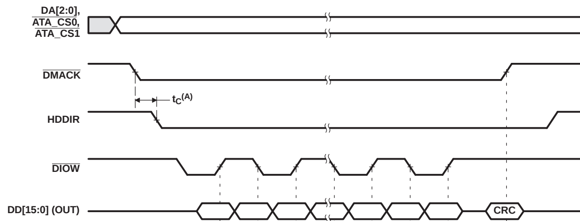
Figure 6-40. ATA/CF HDDIR Multiword DMA Write Transfer Timing
