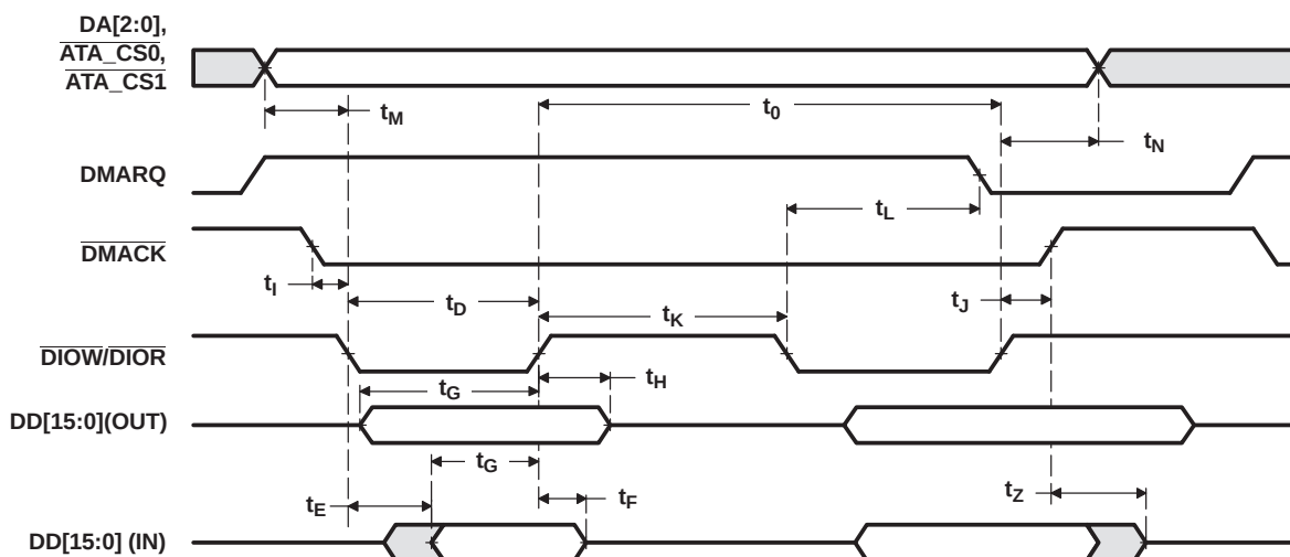
Figure 6-27. ATA/CF Multiword DMA Timing
