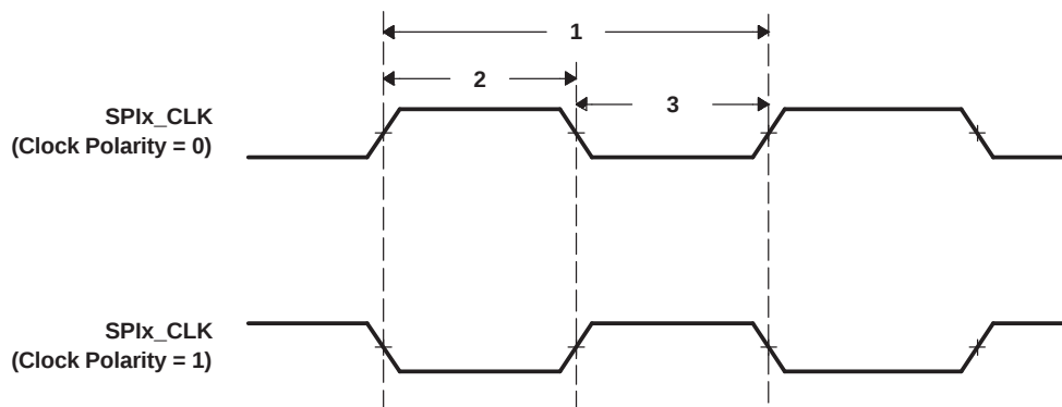
Figure 6-62. SPI_CLK Timing
