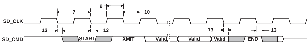
Figure 6-42. MMC/SD/SDIO Host Command Timing
