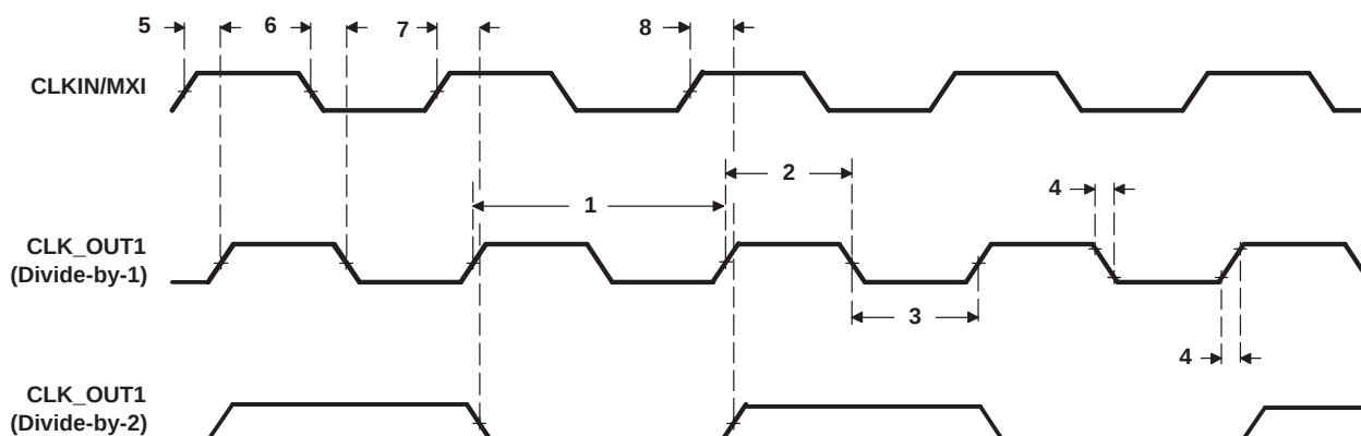
Figure 6-17. CLK_OUT1 Timing
