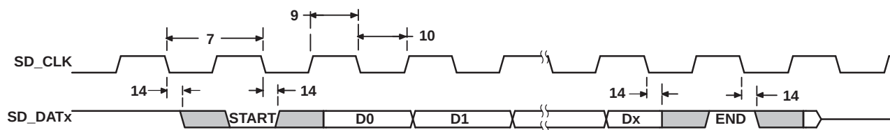
Figure 6-44. MMC/SD/SDIO Host Write Timing
