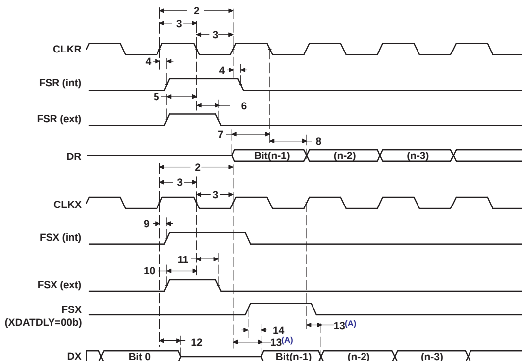
Figure 6-67. ASP Timing
