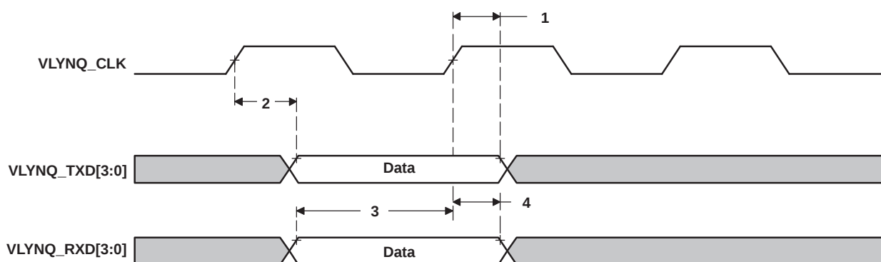
Figure 6-78. VLYNQ Transmit/Receive Timing
