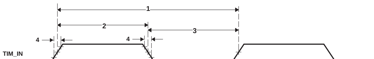
Figure 6-74. Timer Timing
