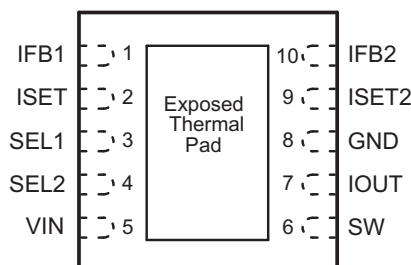
QFN PACKAGE (TOP VIEW)
