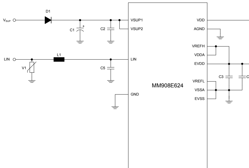
Figure 20. EMC/EMI Recommendations
