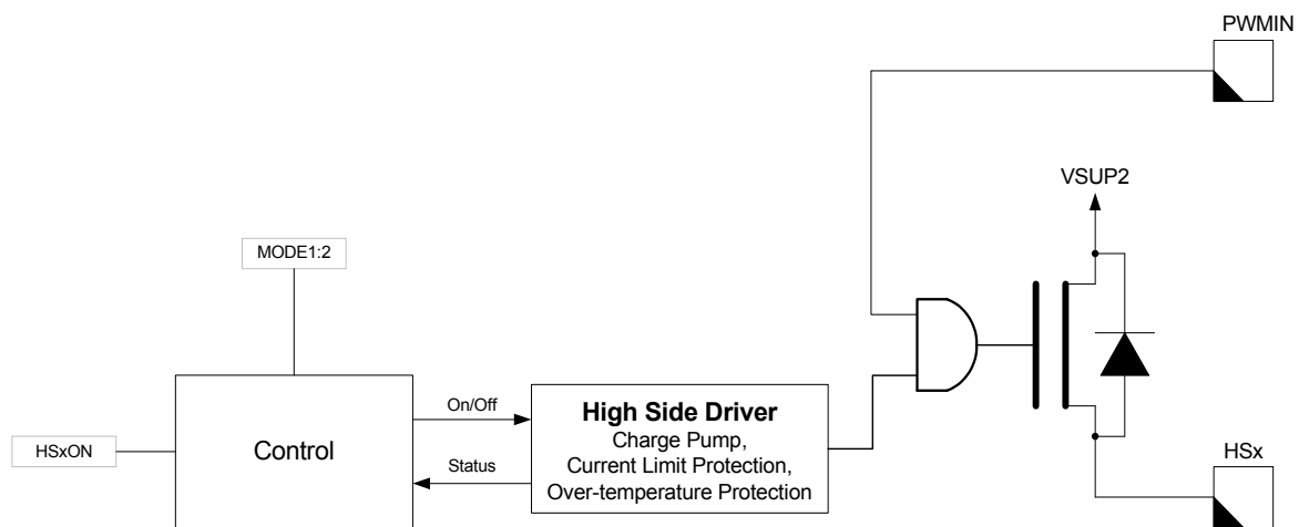
Figure 13. High Side HS1 and HS2 Circuitry
