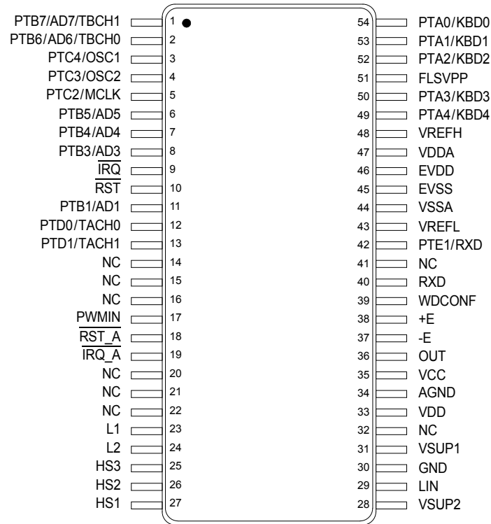
Figure 3. Pin Connections
