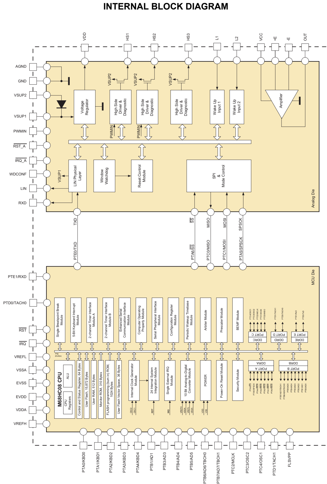
Figure 2. 908E624 Simplified Internal Block Diagram
