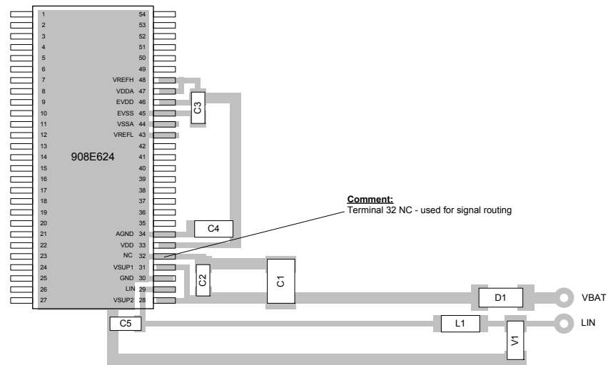
Figure 21. PCB Layout Recommendations
