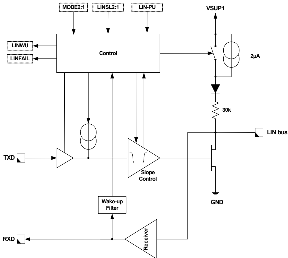
Figure 15. LIN Interface
