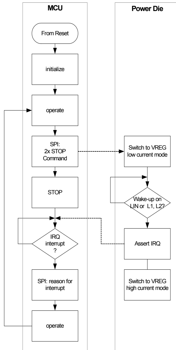
Figure 12. Stop Mode/Wake-up Procedure
