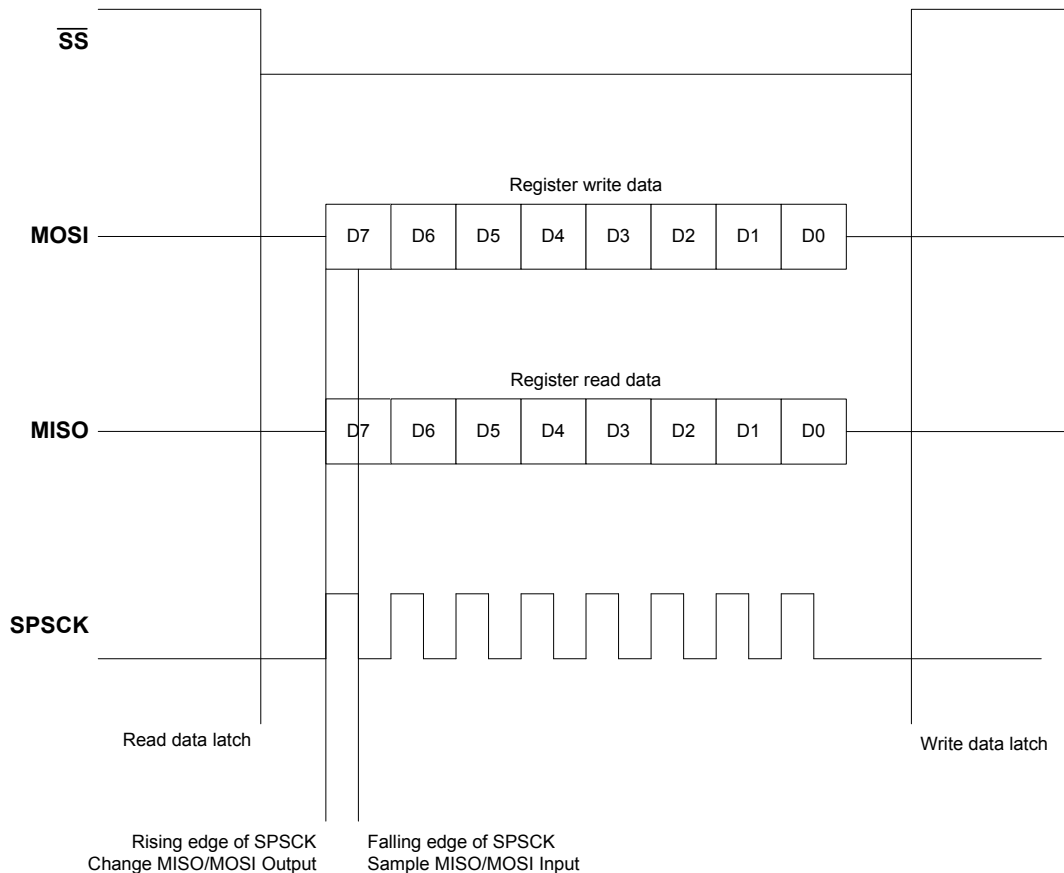
Figure 17. SPI Protocol
