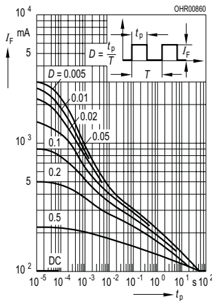
Permissible Pulse Handling Capability I_F = f(\tau) , T_A = 25 \text{ }^\circ\text{C} duty cycle D = parameter
