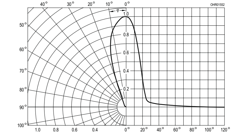
Radiation Characteristics, I_{rel} = f(\phi)
