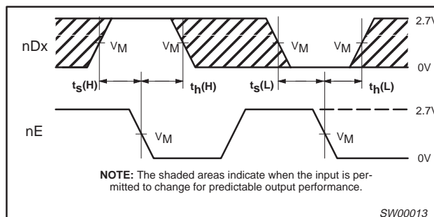
Waveform 3. Data Setup and Hold Times
