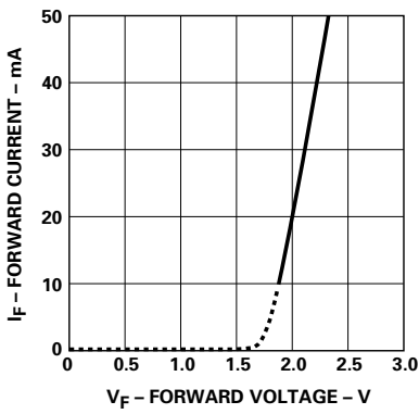
Figure 2. AllnGaP forward current vs. forward voltage.
