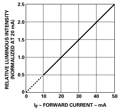
Figure 4. AllnGaP relative luminous intensity vs. forward current.
