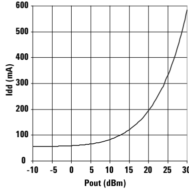
Figure 2. Total Idd vs Pout
