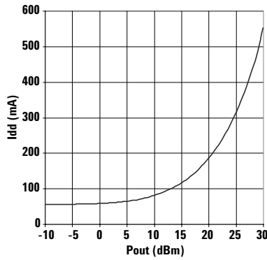
Figure 12. Total Idd vs Pout
