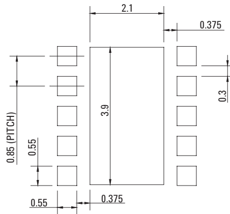
Figure 16. PCB land pattern (dimensions in mm)
