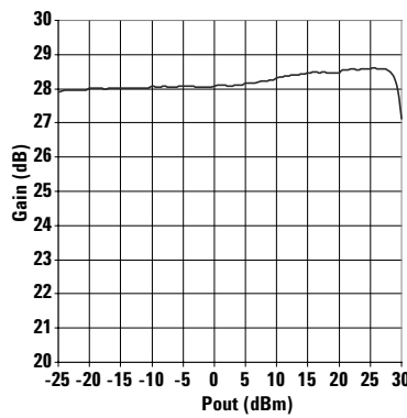
Figure 15. Gain vs Pout
