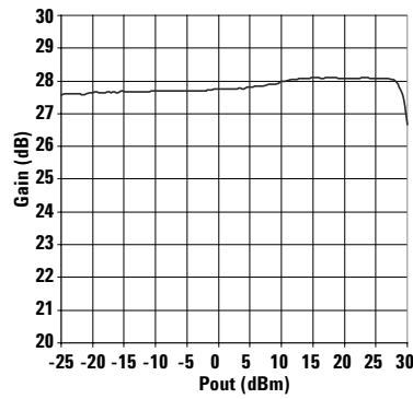
Figure 5. Gain vs Pout
