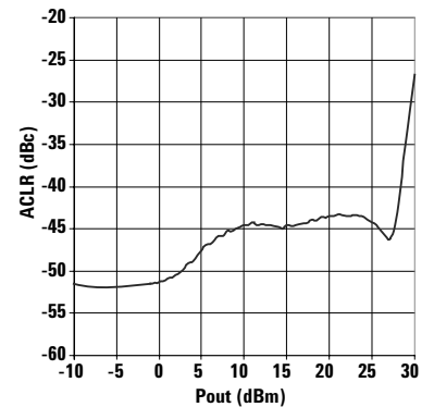
Figure 8. ACLR1 vs Pout
