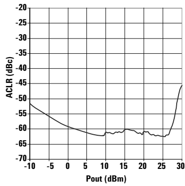
Figure 9. ACLR2 vs Pout
