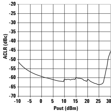
Figure 4. ACLR2 vs Pout
