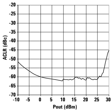
Figure 14. ACLR2 vs Pout
