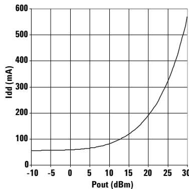
Figure 7. Total Idd vs Pout
