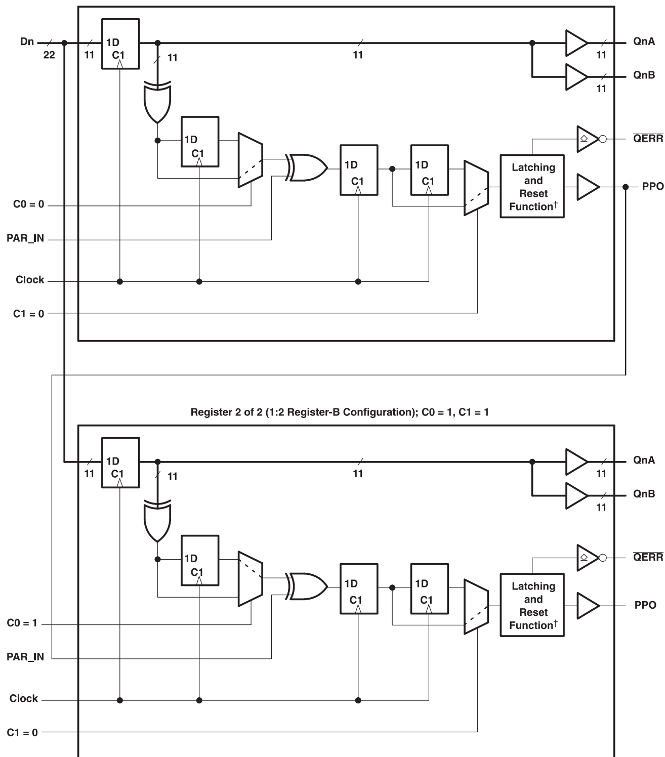
Register 1 of 2 (1:2 Register-A Configuration): C0 = 0, C1 = 1
