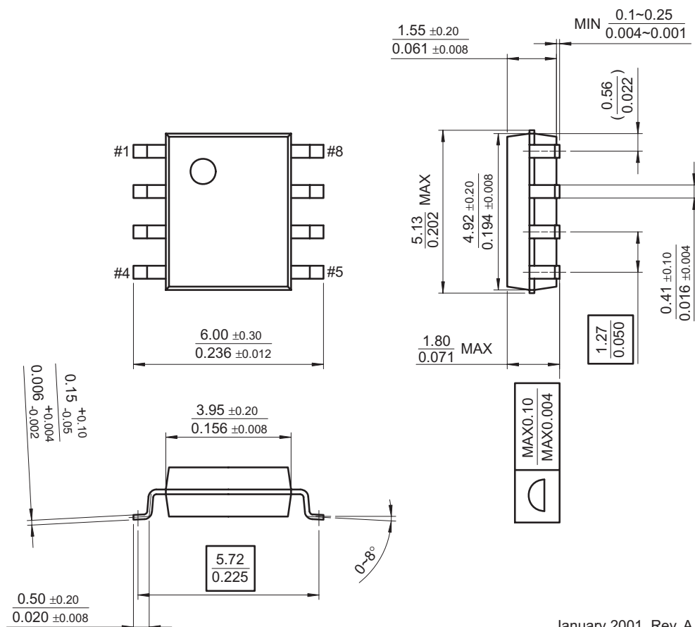
Figure 27. 8-Lead Small Outline Package (SOP)
