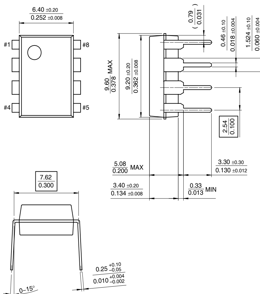
Figure 28. 8-Lead Dual In-Line Package (DIP)
