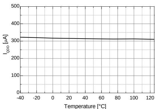
Figure 7. V_{DD} Quiescent Current vs. Temperature
