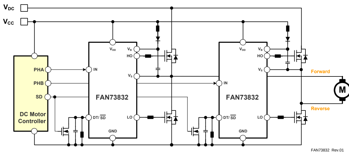
Figure 2. Application Circuit for Full-Bridge DC Motor Driver
