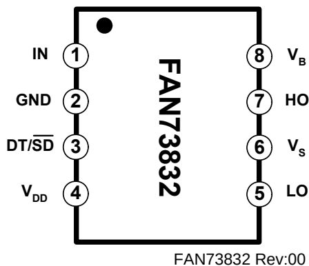
Figure 4. Pin Configuration (Top View)
