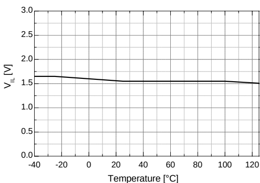
Figure 13. Logic Input Low Voltage vs. Temperature
