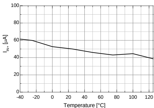
Figure 11. Logic Input Current vs. Temperature
