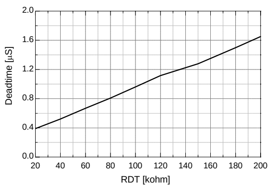
Figure 20. R DT vs. Dead-Time
