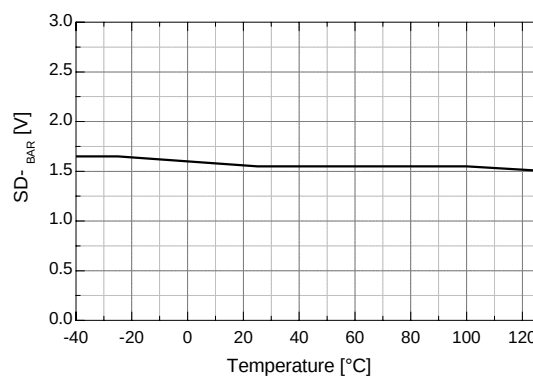
Figure 15. SD Negative Threshold vs. Temperature
