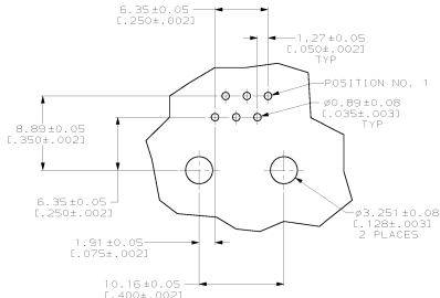
PRINTED CIRCUIT BOARD LAYOUT NONCOMPONENT SIDE SHOWN
