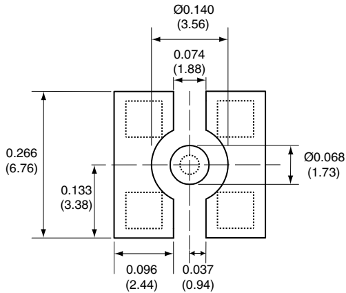
RECOMMENDED FOOTPRINT
