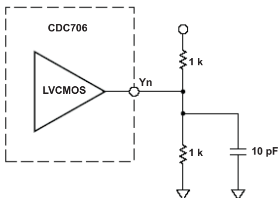
Figure 1. Test Load
