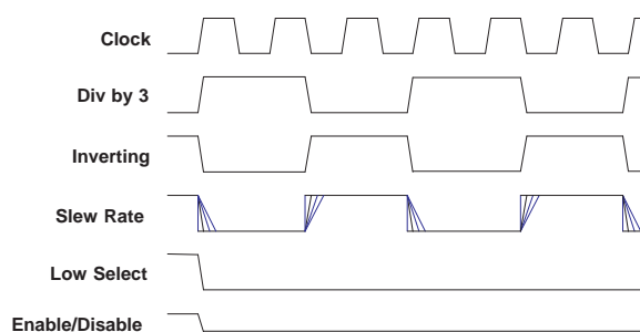
Figure 25. Example for Output Waveforms
