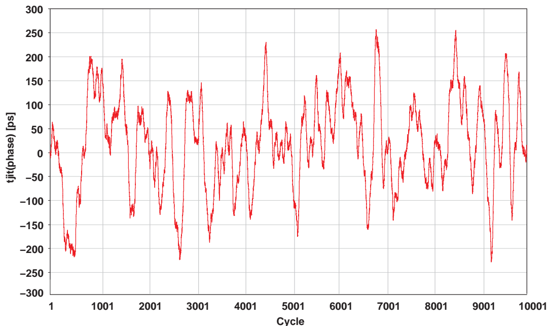
Figure 28. Snapshot of Phase Jitter
