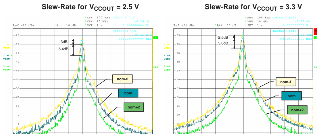
Figure 21. EMI Reduction vs Slew-Rate and V_{ccout}
