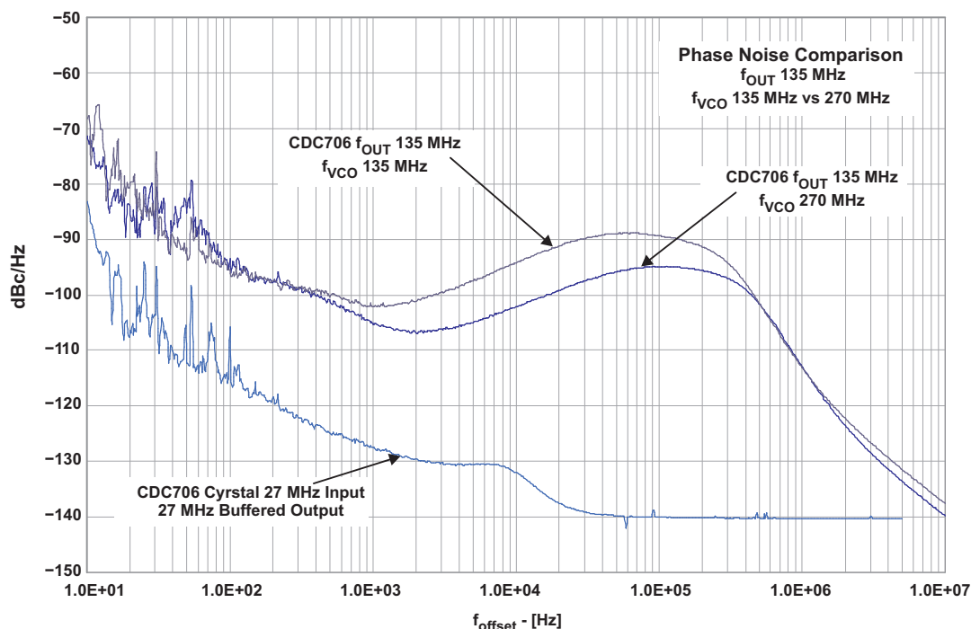
Figure 32. Phase Noise Characteristic - f_{\text{offset}} - Hz
