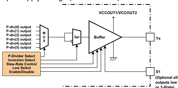
Figure 24. Block Diagram of Output Architecture
