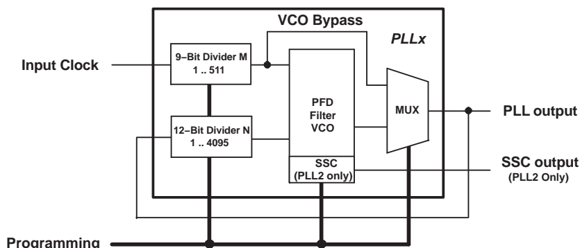
Figure 18. PLL Architecture
