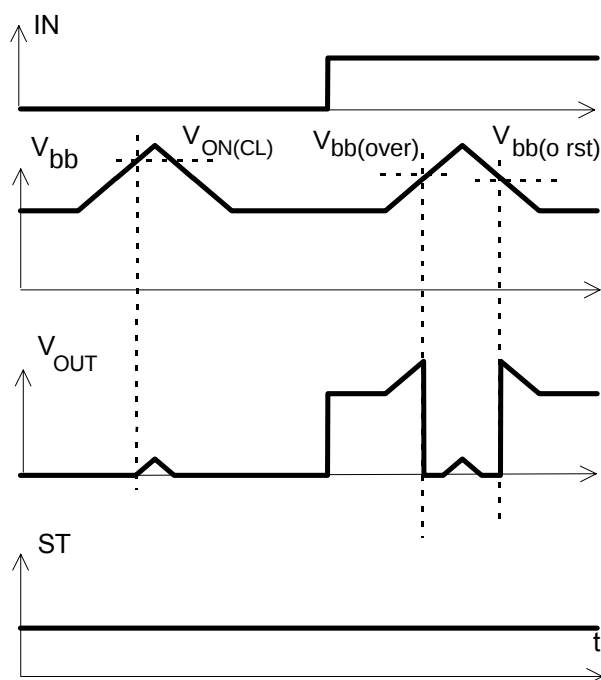
Figure 7a: Overvoltage:
