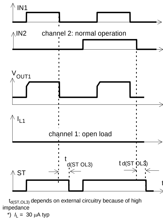
Figure 6a: Undervoltage:
