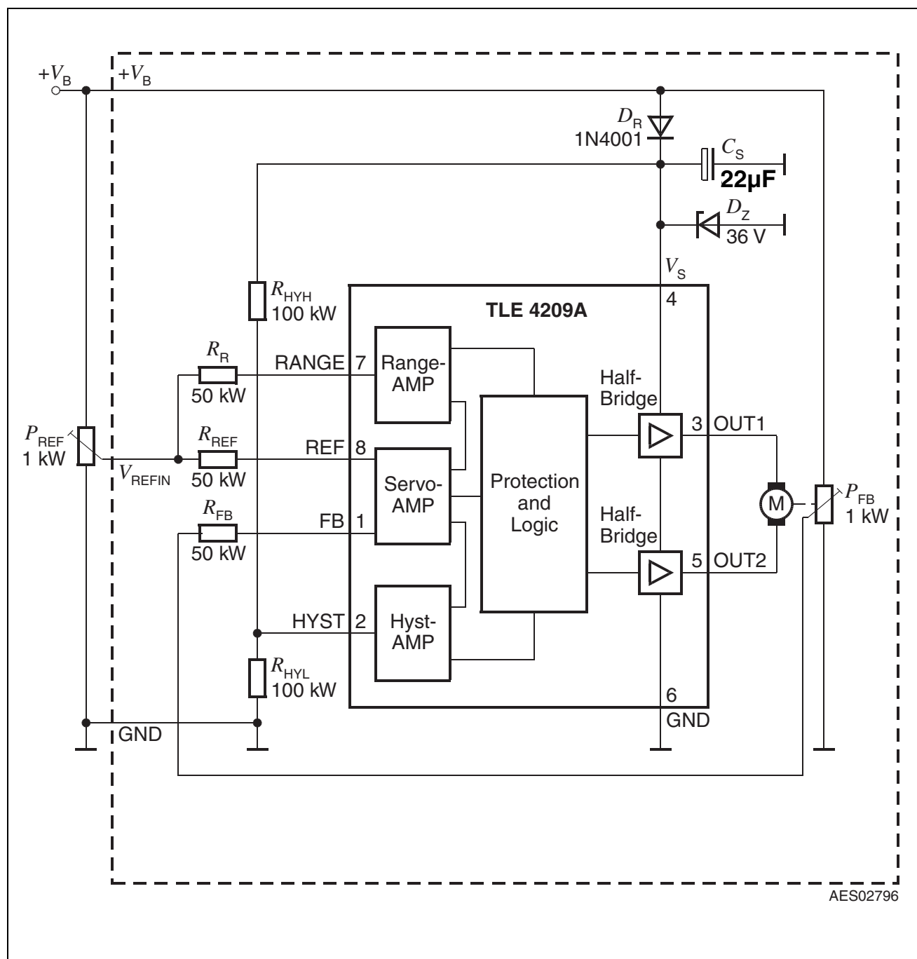
Figure 3 Application Circuit
