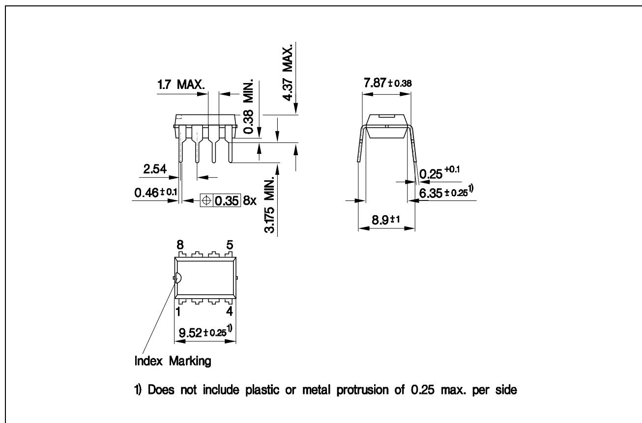
Figure 6 PG-DIP-8-4 (Plastic Dual In-line Package)
