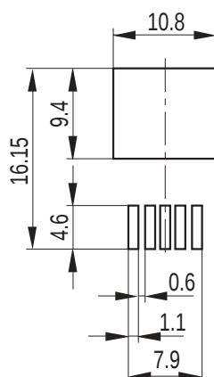
Figure 8 Foot Print for P-TO263-5-1 (Plastic Transistor Single Outline)
