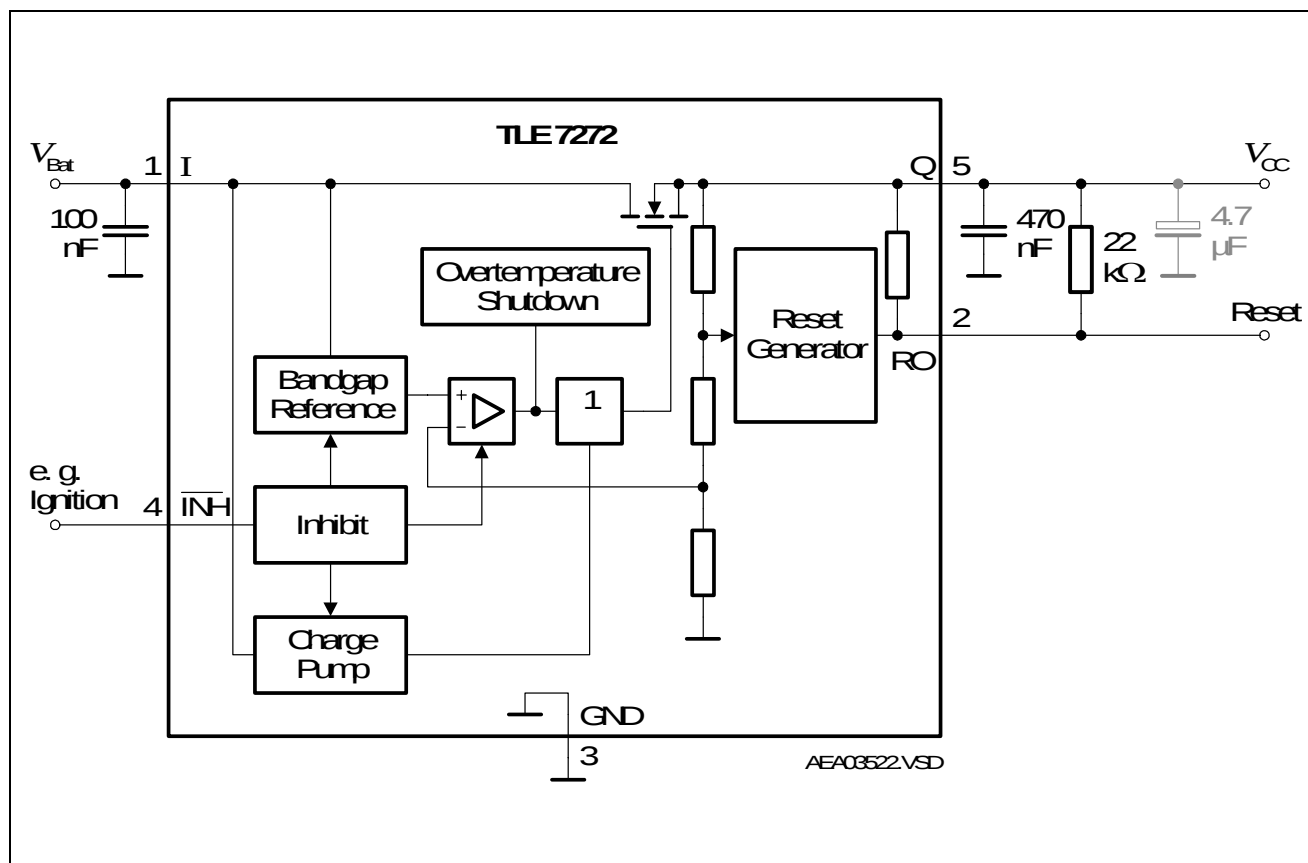
Figure 3 Application Diagram
