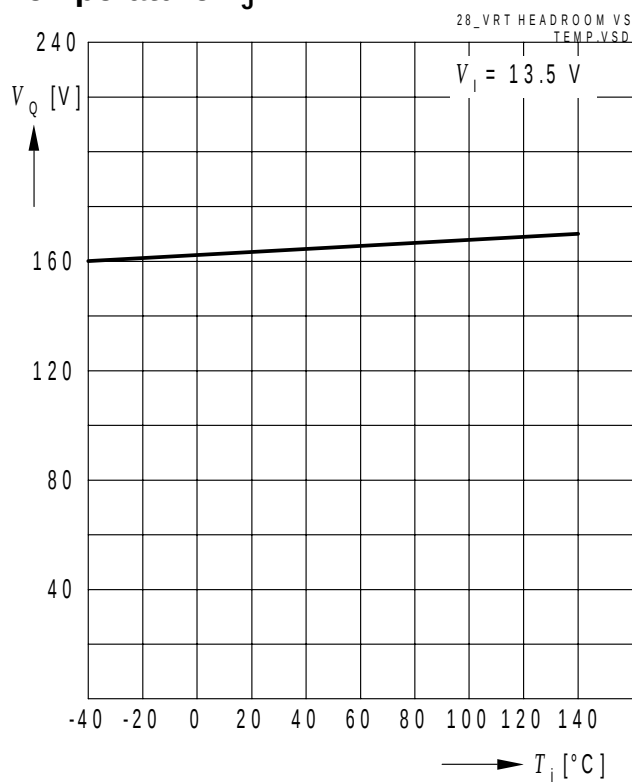
Reset Headroom versus Junction Temperature T_j
