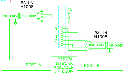
INSERTION LOSS TEST CIRCUIT FIGURE 4
