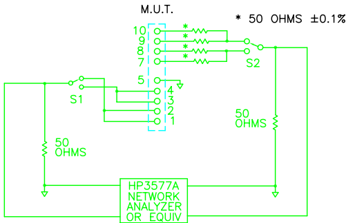
COMMON MODE REJECTION FIGURE 8
