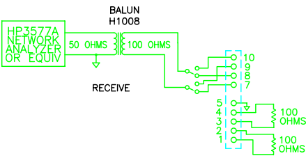
RETURN LOSS TEST CIRCUIT FIGURE 6
