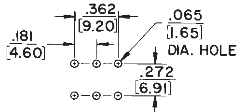
RECOMMENDED PC BOARD LAYOUT (Component Side)
