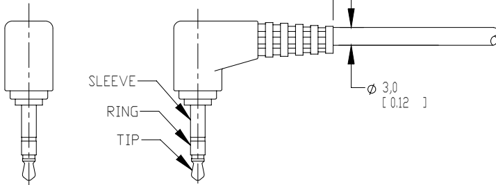
RA 2.5mm 3 CONDUCTOR PLUG
