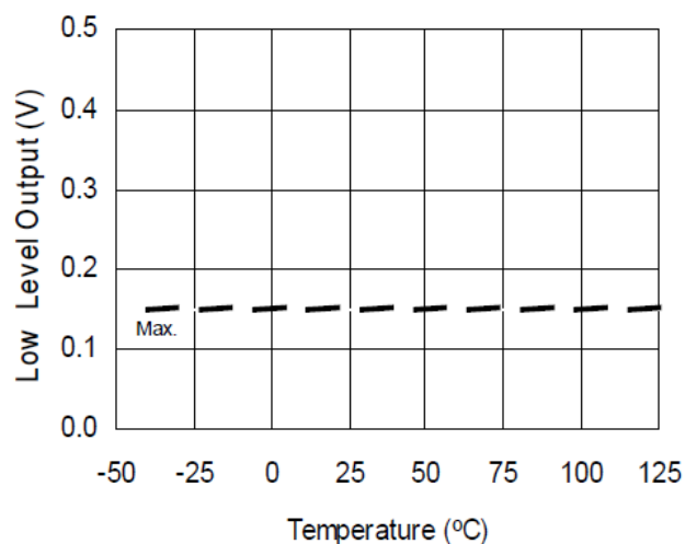
Figure 11A. Low Level Output vs. Temperature
