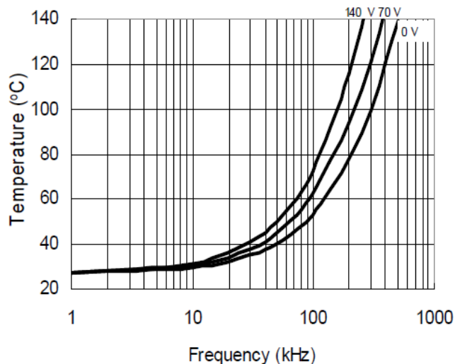
Figure 36. IRS21864S vs. Frequency (IRFPE50) R_{gate} = 10\Omega , V_{CC} = 15V
