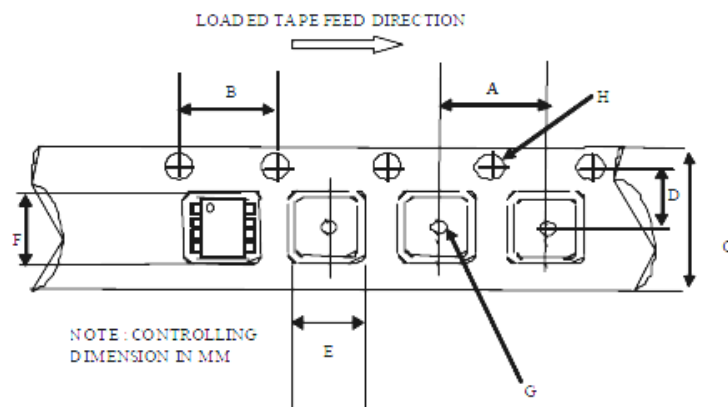
CARRIER TAPE DIMENSION FOR 14SOICN
