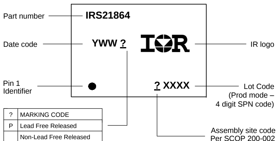
14-Lead PDIP
