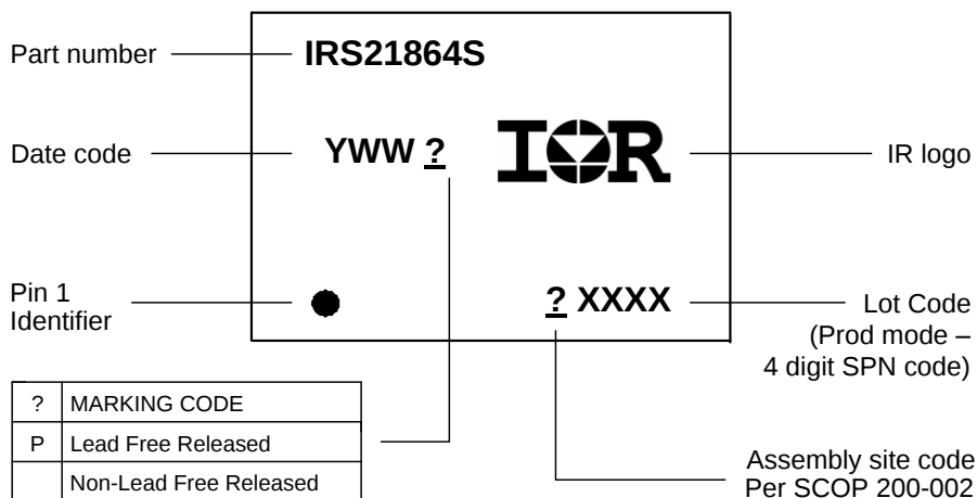
14-Lead SOIC
