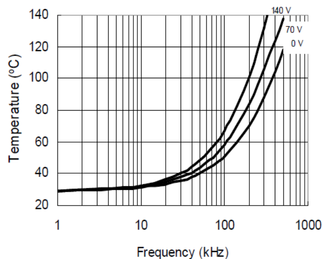
Figure 24. IRS2186 vs. Frequency (IRFPE50) R_{gate} = 10\Omega , V_{CC} = 15V
