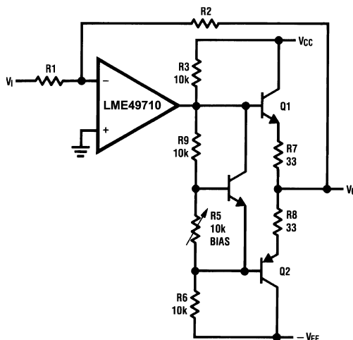
Figure 91. Line Driver
