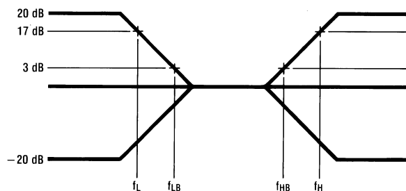
Figure 92. Tone Control
