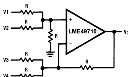
Figure 86. Adder/Subtractor
