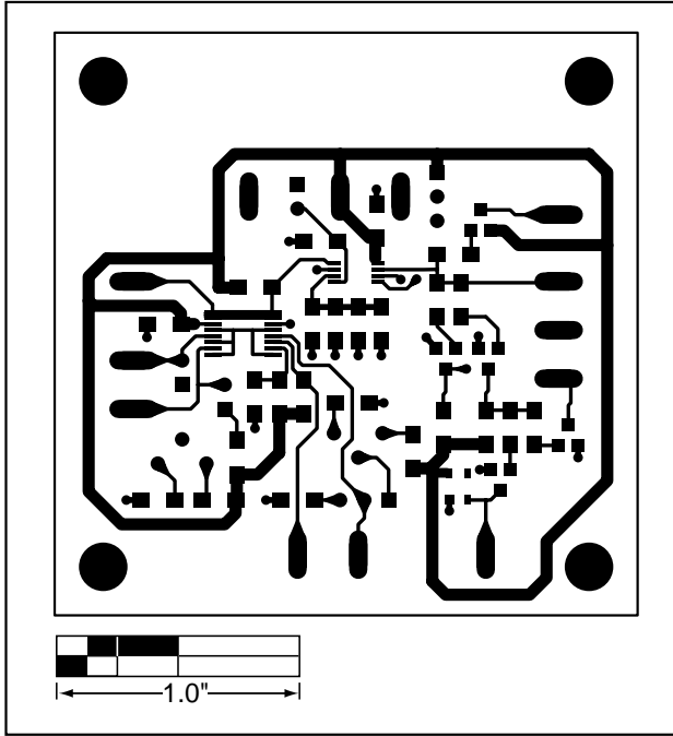
Figure 3. SUPEVKIT PC Board Layout—Component Side
