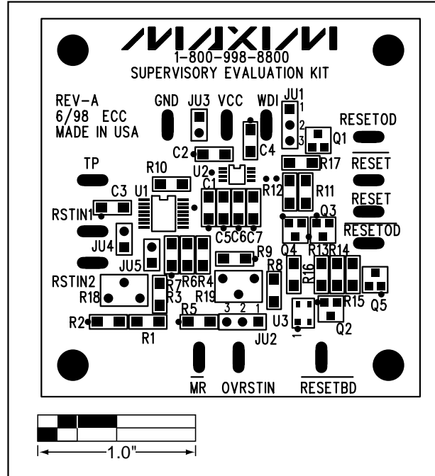
Figure 2. SUPEVKIT Component Placement Guide— Component Side
