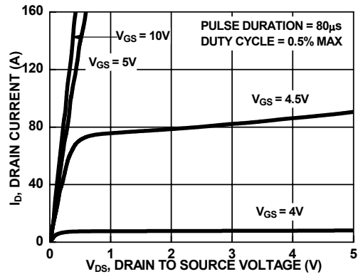
Figure 8. Saturation Characteristics
