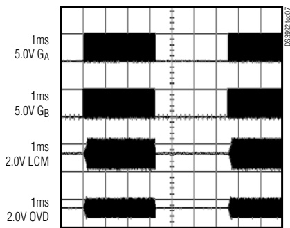
BURST DIMMING AT 150Hz AND 50%
