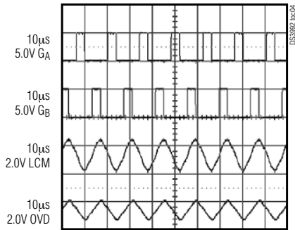
TYPICAL OPERATION AT 16V
