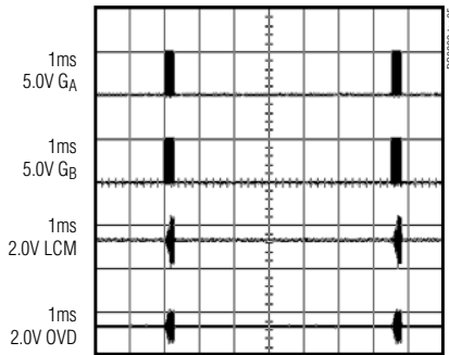
BURST DIMMING AT 150Hz AND 10%
