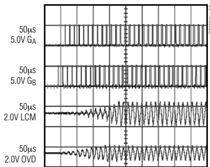
SOFT-START AT VINV = 16V
