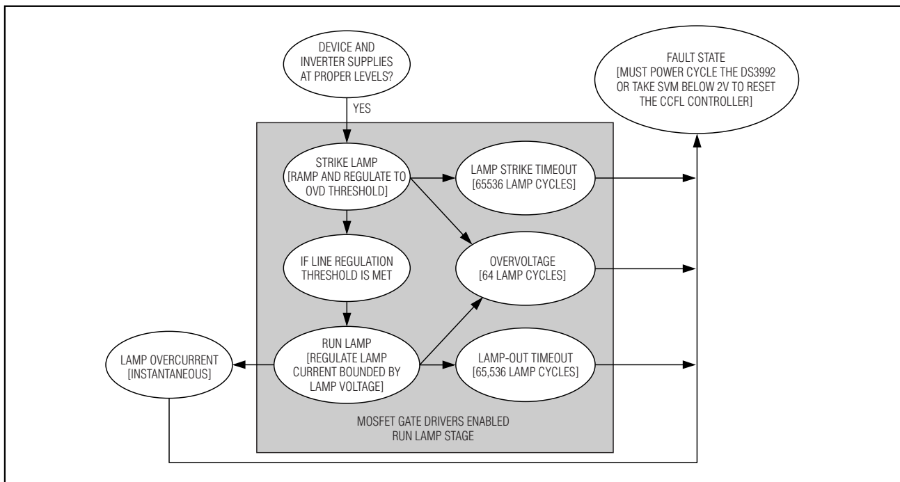
Figure 4. Fault-Handling Flowchart
