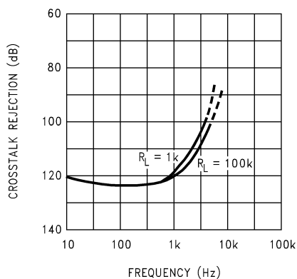
Crosstalk Rejection vs Frequency
