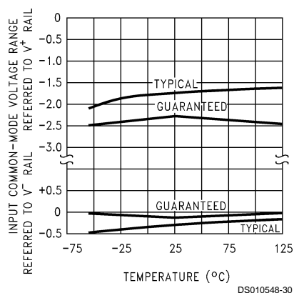
Input Common-Mode Voltage Range vs Temperature
