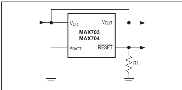
Figure 6. \overline{\text{RESET}} Valid to Ground Circuit
