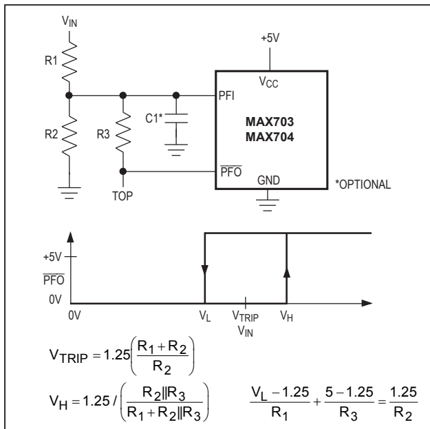
Figure 7. Adding Hysteresis to the Power-Fail Comparator
