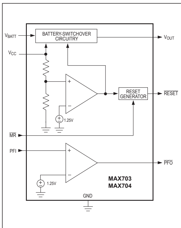
Figure 1. Block Diagram
