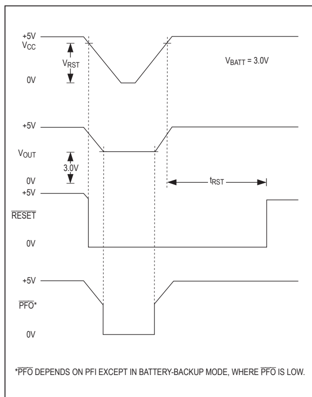
Figure 2. Timing Diagram
