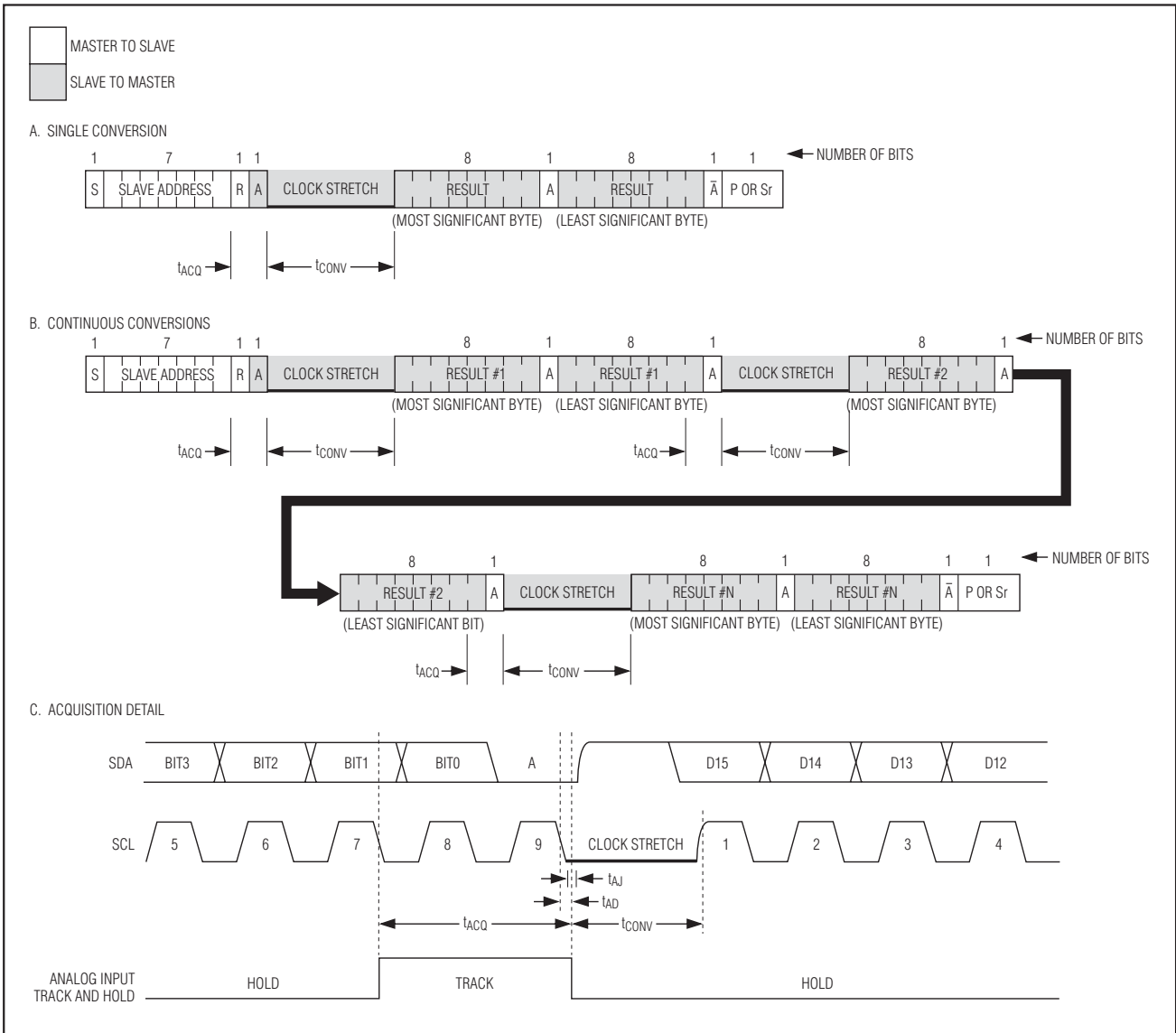
Figure 11. Read Cycle
