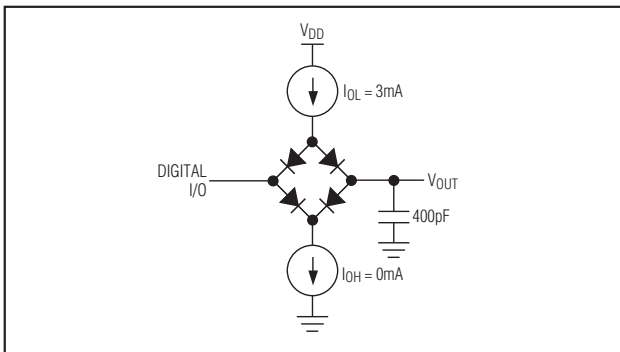
Figure 2. Load Circuit
