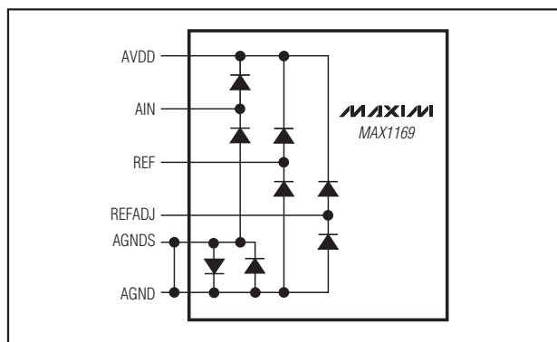
Figure 6. Internal Protection Diodes
