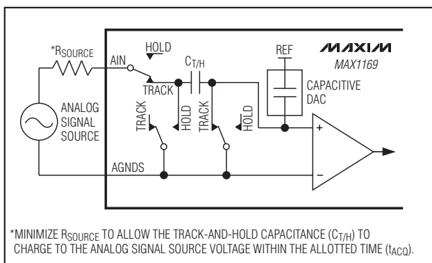
Figure 5. Equivalent Input Circuit
