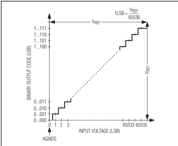
Figure 14. Unipolar Transfer Function
