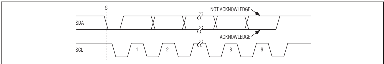
Figure 8. Acknowledge Bits
