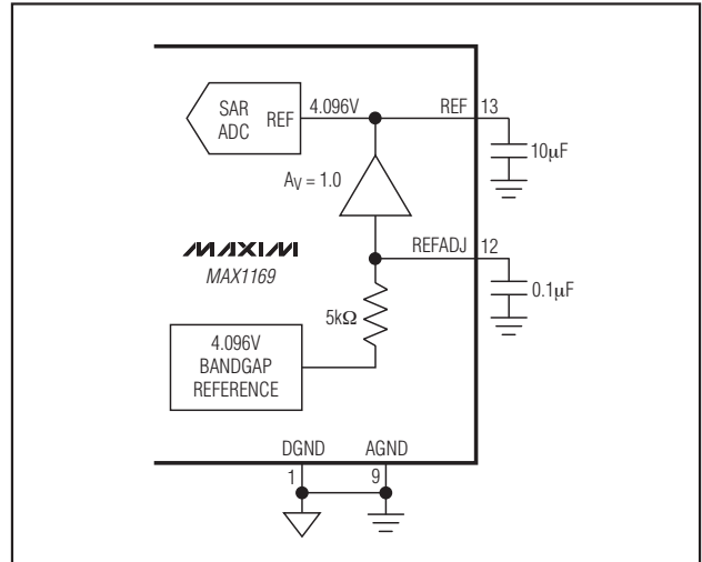
Figure 12. Internal Reference
