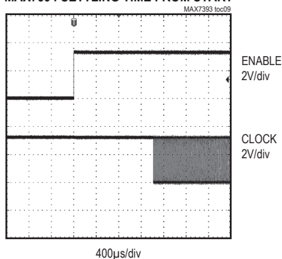
MAX7394 SETTLING TIME FROM START
