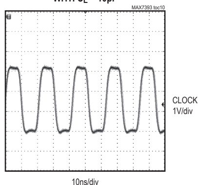
CLOCK OUTPUT WAVEFORM WITH C_L = 10pF
