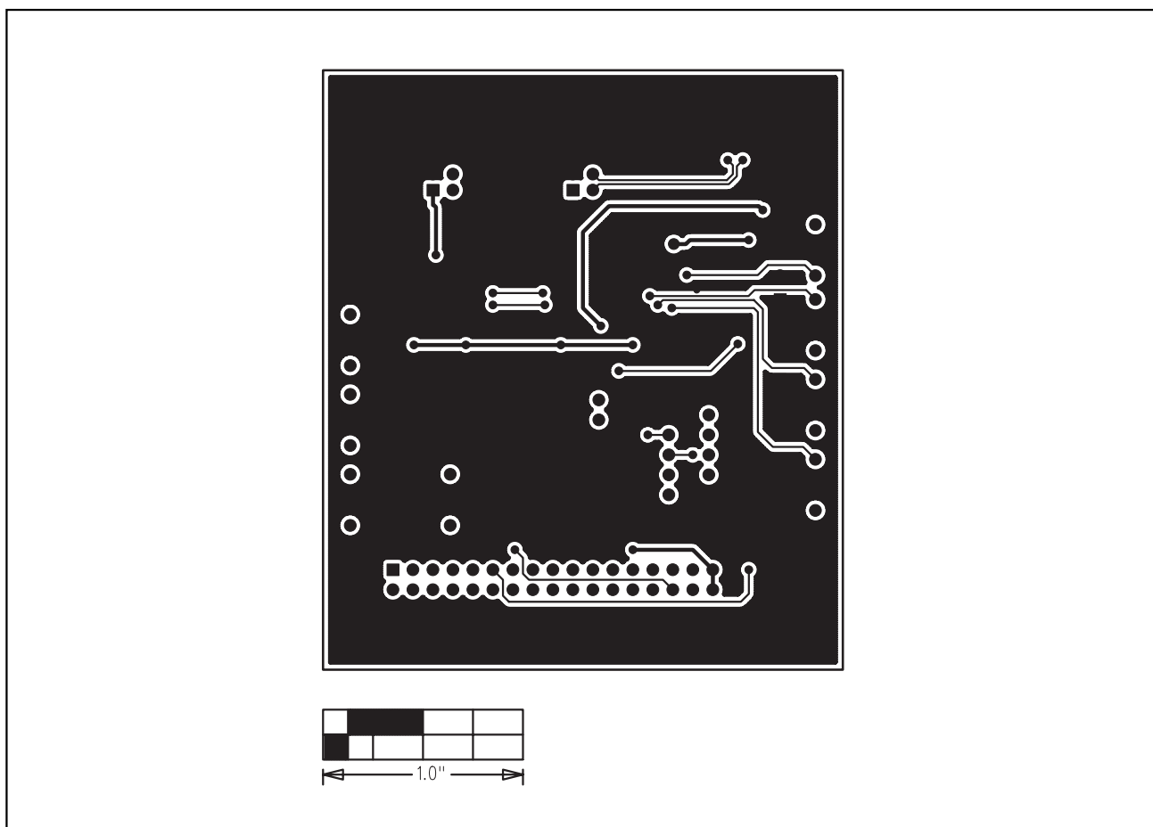
Figure 5. MAX3421 EV Kit-1 PCB Layout—Solder Side
