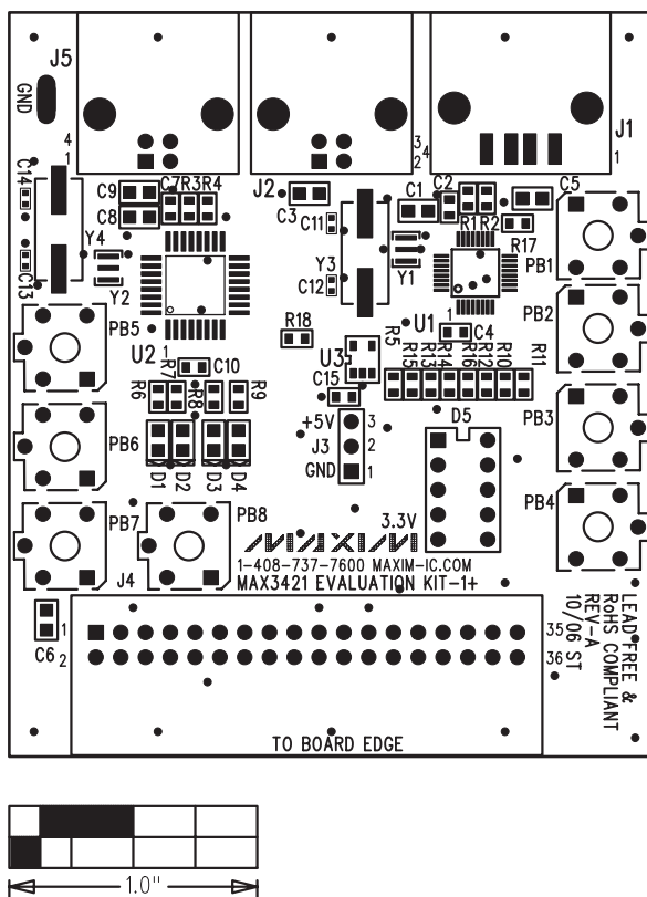
Figure 3. MAX3421 EV Kit-1 Component Placement Guide—Component Side
