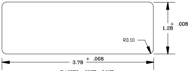
PANEL CUT-OUT
