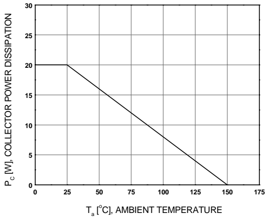
Figure 9. Power Derating
