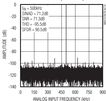
FFT PLOT (MAX1278)
