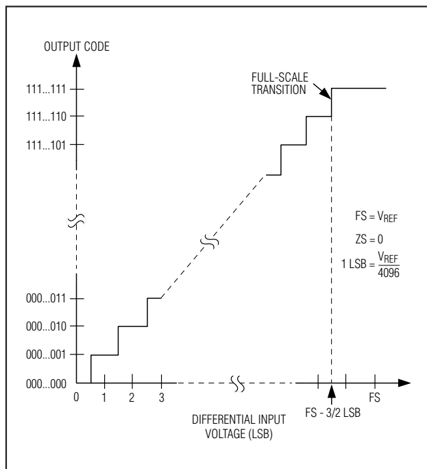
Figure 8. Unipolar Transfer Function (MAX1276 Only)
