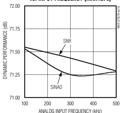
DYNAMIC PERFORMANCE vs. INPUT FREQUENCY (MAX1278)
