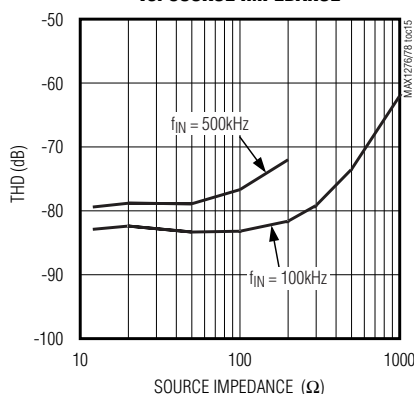
TOTAL HARMONIC DISTORTION vs. SOURCE IMPEDANCE
