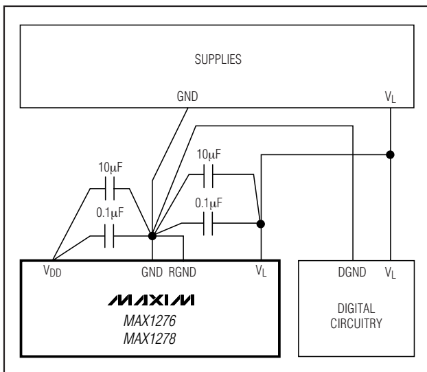
Figure 20. Power-Supply Grounding Condition
