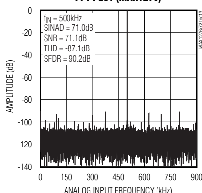
FFT PLOT (MAX1276)
