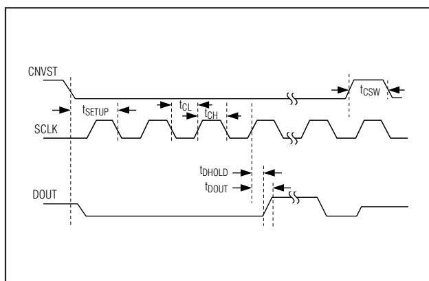
Figure 1. Detailed Serial-Interface Timing
