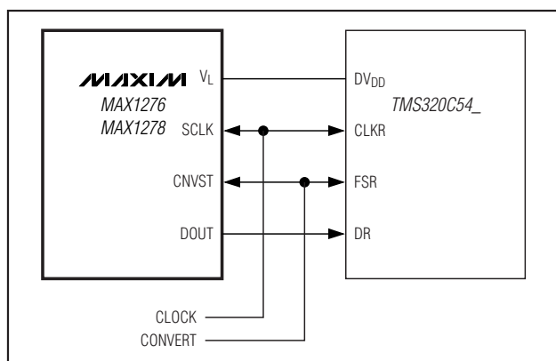
Figure 16. Interfacing to the TMS320C54_ External Clocks
