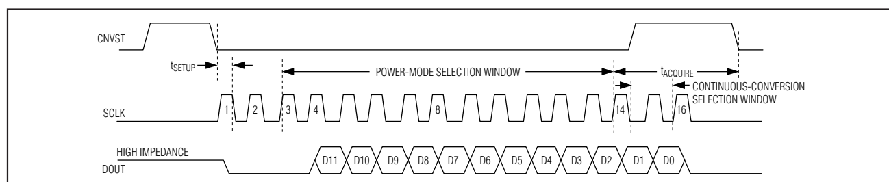
Figure 5. Interface-Timing Sequence
