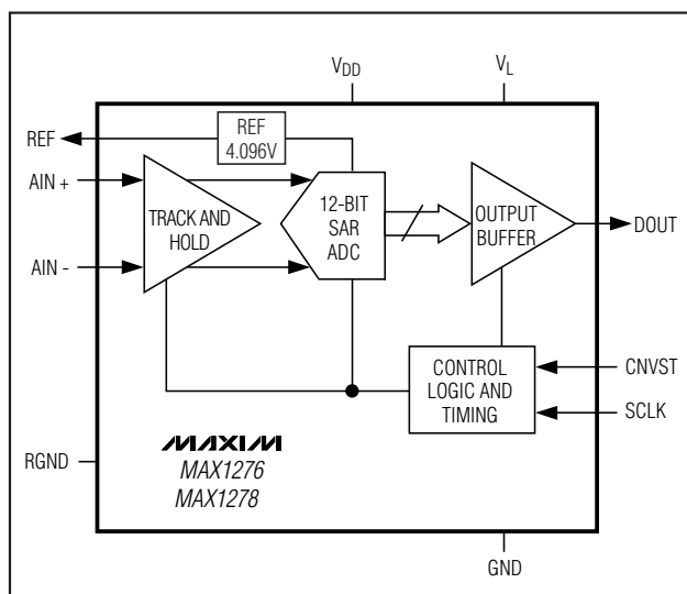
Figure 3. Functional Diagram
