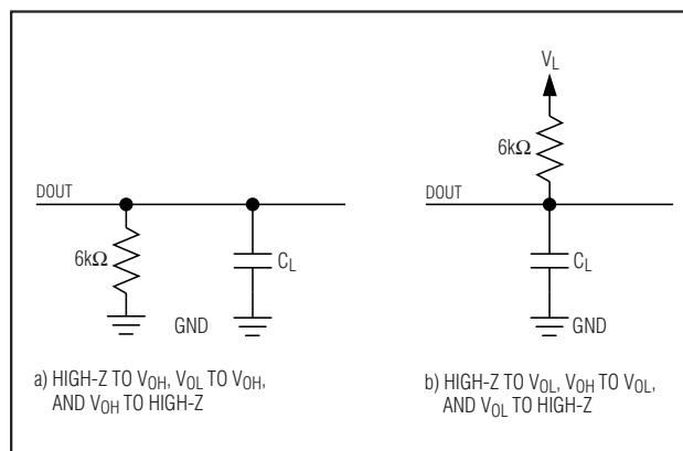
Figure 2. Load Circuits for Enable/Disable Times
