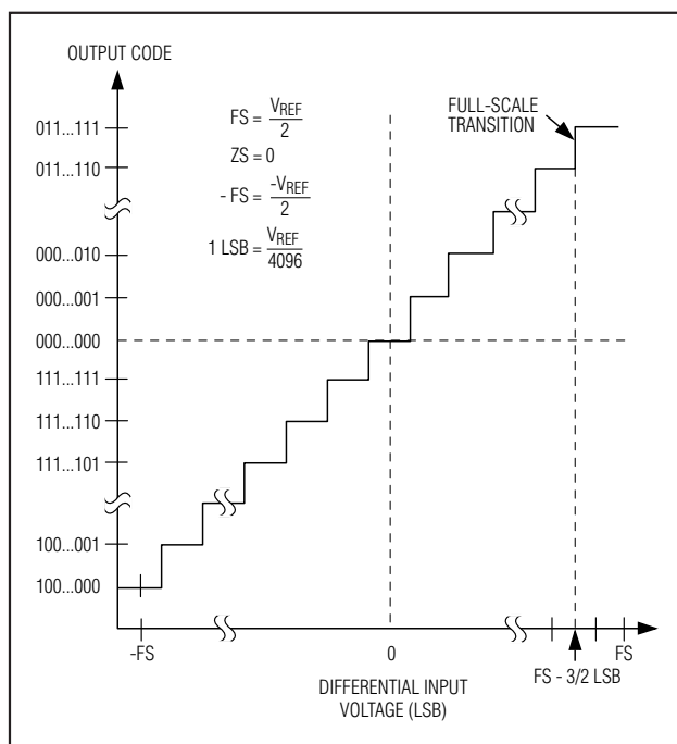
Figure 9. Bipolar Transfer Function (MAX1278 Only)
