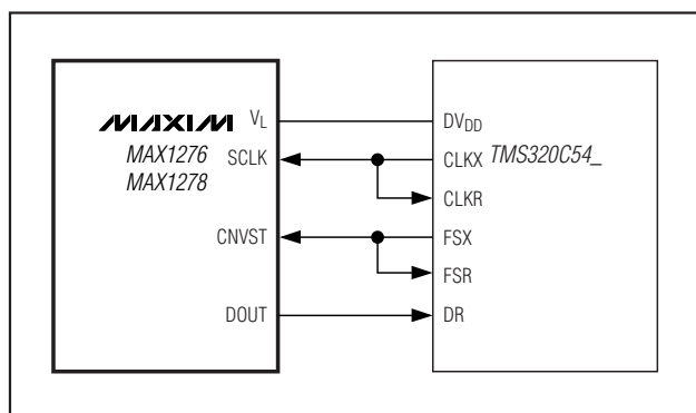
Figure 15. Interfacing to the TMS320C54_ Internal Clocks
