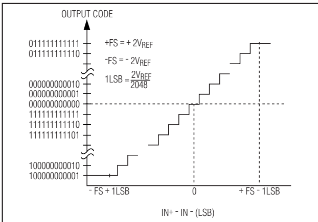
Figure 5. Bipolar Transfer Function
