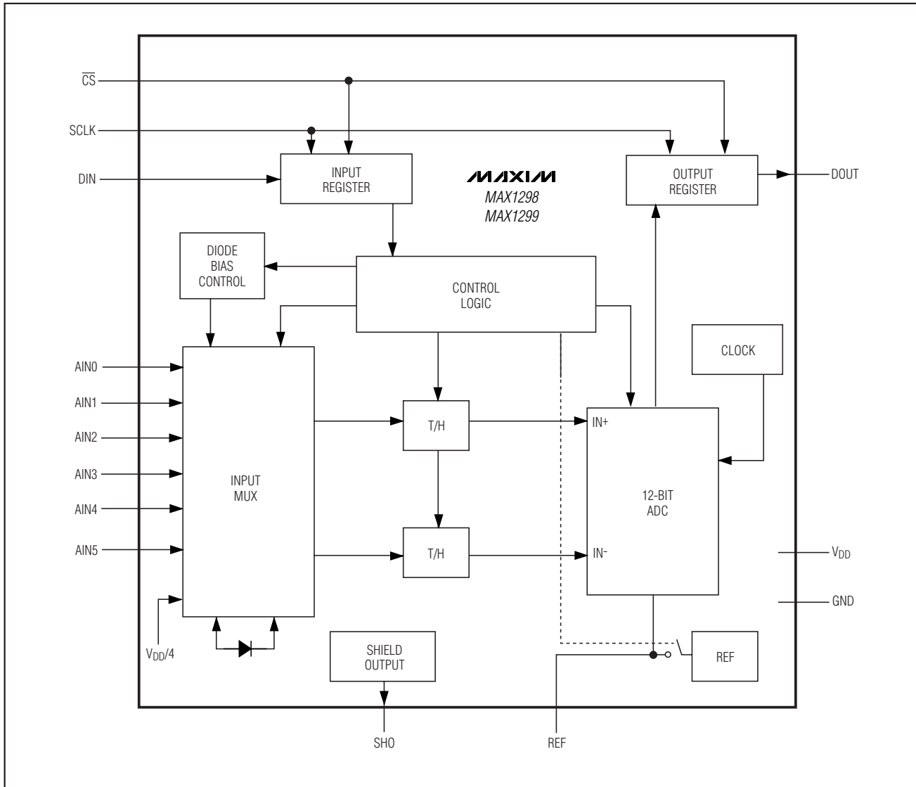
Figure 1. Functional Diagram
