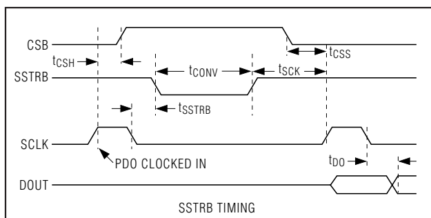
Figure 6. Detailed SSTRB Timing
