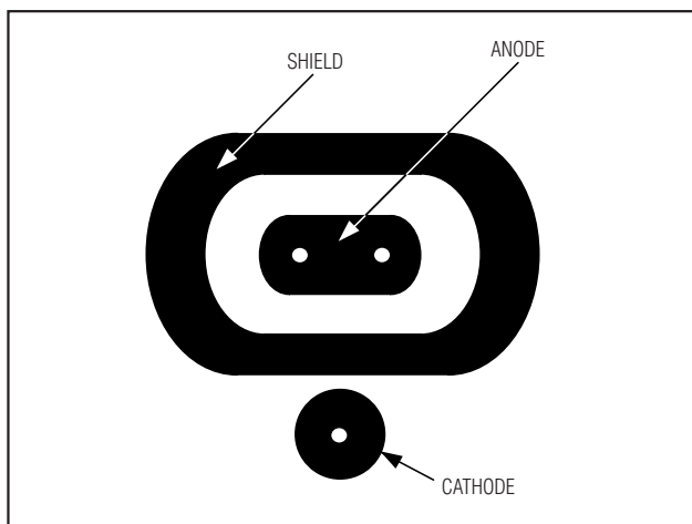
Figure 8. Remote Diode Shielding for PC Boards
