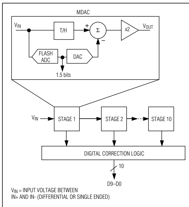
Figure 1. Pipelined Architecture—Stage Blocks
