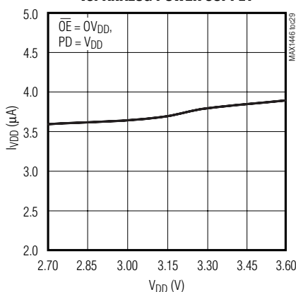
ANALOG POWER-DOWN CURRENT vs. ANALOG POWER SUPPLY
