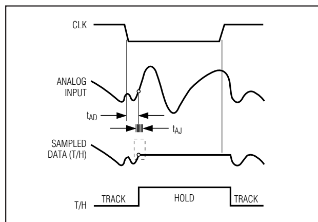
Figure 12. T/H Aperture Timing
