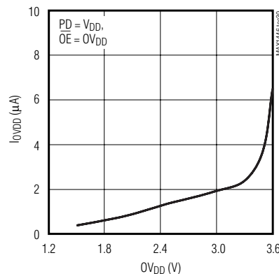
DIGITAL POWER-DOWN CURRENT vs. DIGITAL POWER SUPPLY
