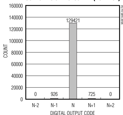
OUTPUT NOISE HISTOGRAM (DC INPUT)
