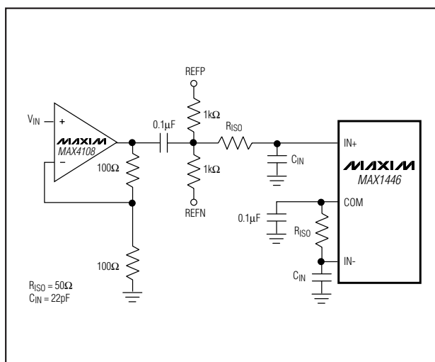
Figure 9. Single-Ended AC-Coupled Input
