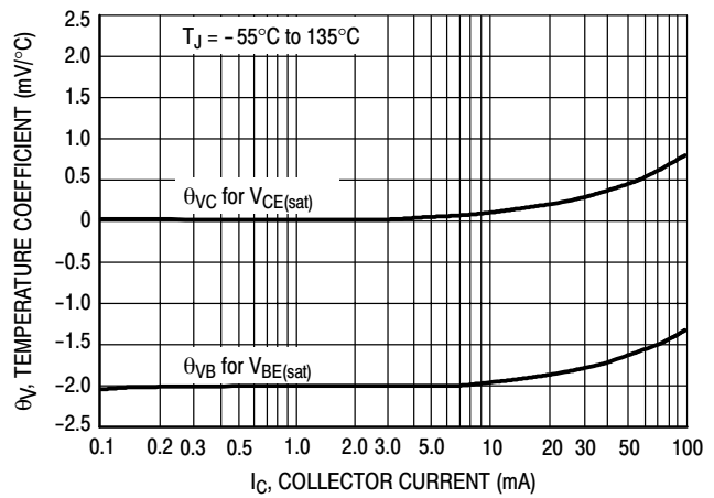
Figure 5. Temperature Coefficients
