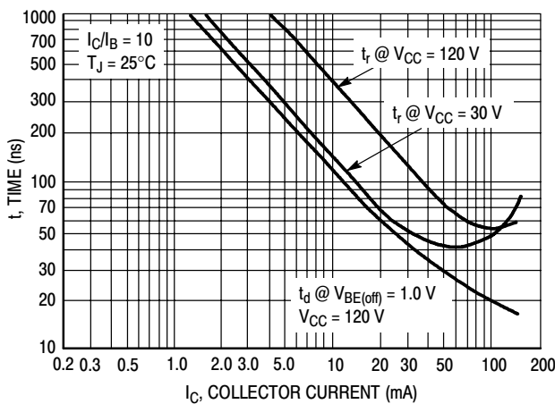
Figure 8. Turn-On Time
