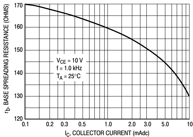
Figure 4. Base Spreading Resistance
