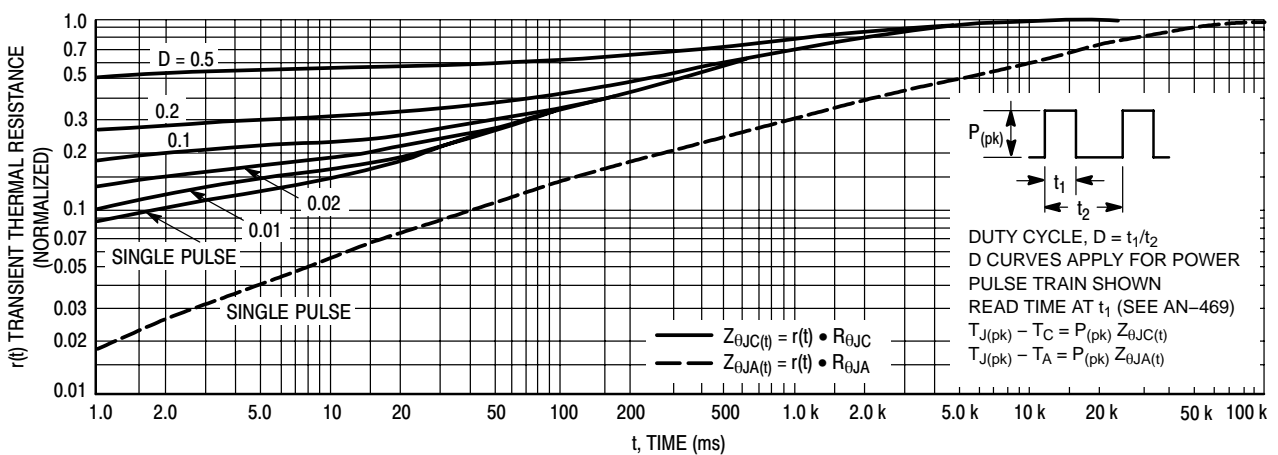
Figure 5. Thermal Response
