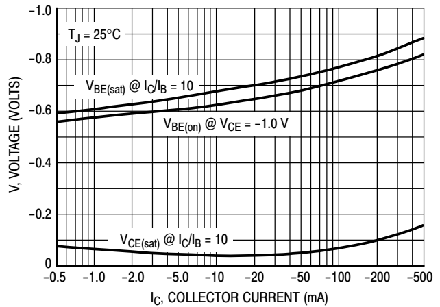
Figure 11. "On" Voltages
