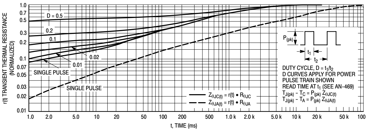
Figure 5. Thermal Response
