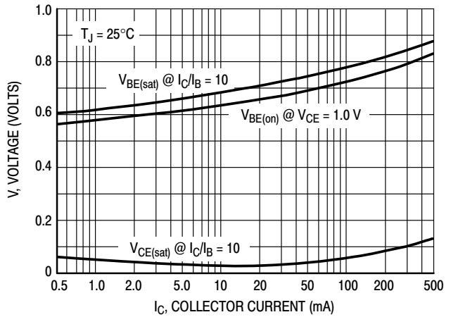
Figure 7. "On" Voltages
